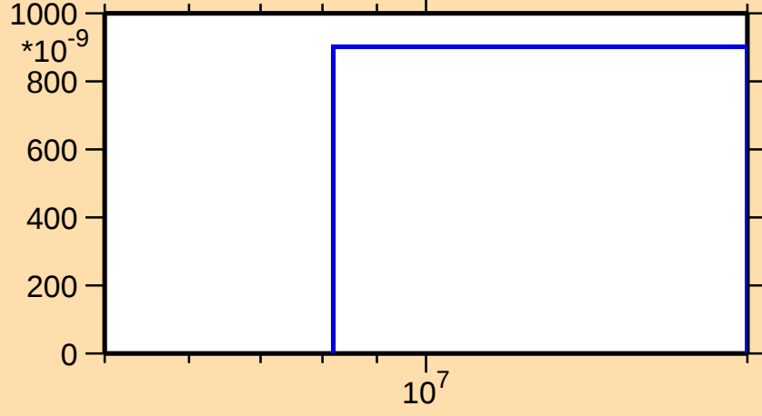
\sigma vs. E for ^{121}\text{Cd}(n,t)
