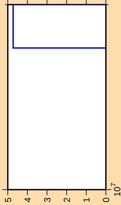
\Delta\sigma/\sigma vs. E for ^{121}\text{Cd}(n,2np)
