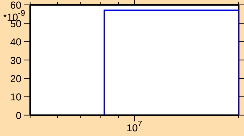
\sigma vs. E for ^{121}\text{Cd}(n,n\alpha)
