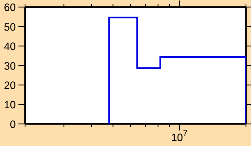
\Delta\sigma/\sigma vs. E for ^{121}\text{Cd}(n,2n)
