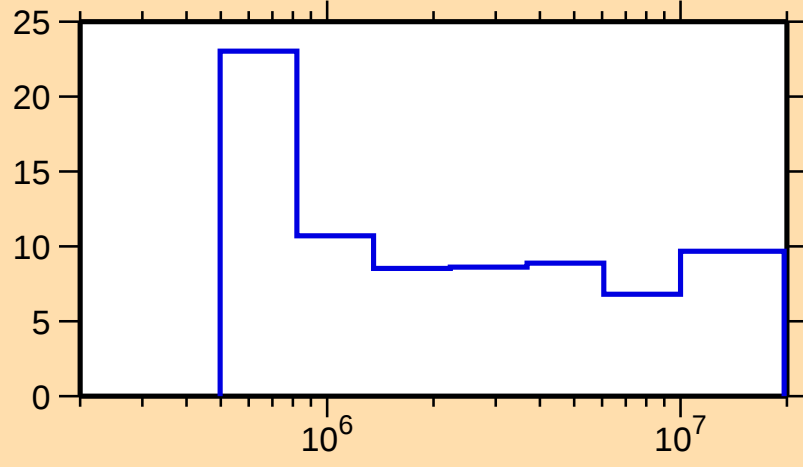
\Delta\sigma/\sigma vs. E for ^{127}\text{Ce}(n,n\text{onel.})
