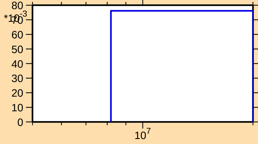
\sigma vs. E for ^{127}\text{Ce}(n,2n)
