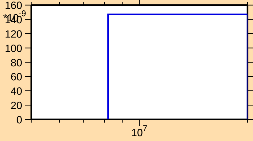
\sigma vs. E for ^{127}\text{Ce}(n,\text{pt})
