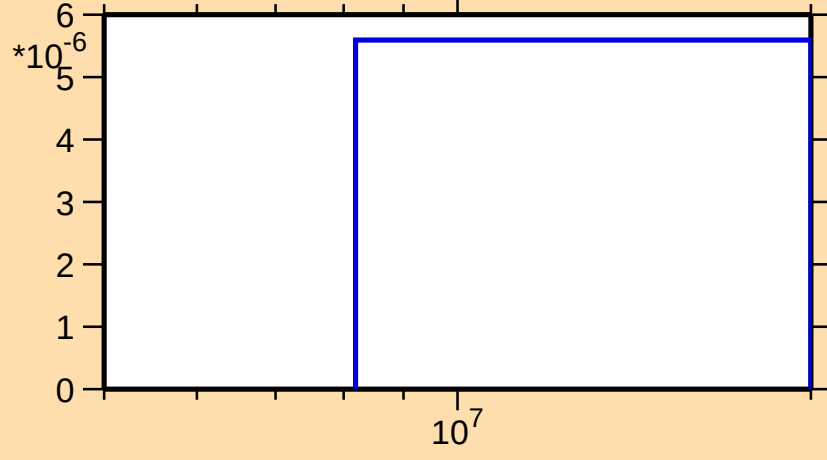
\sigma vs. E for ^{127}\text{Ce}(n,2np)
