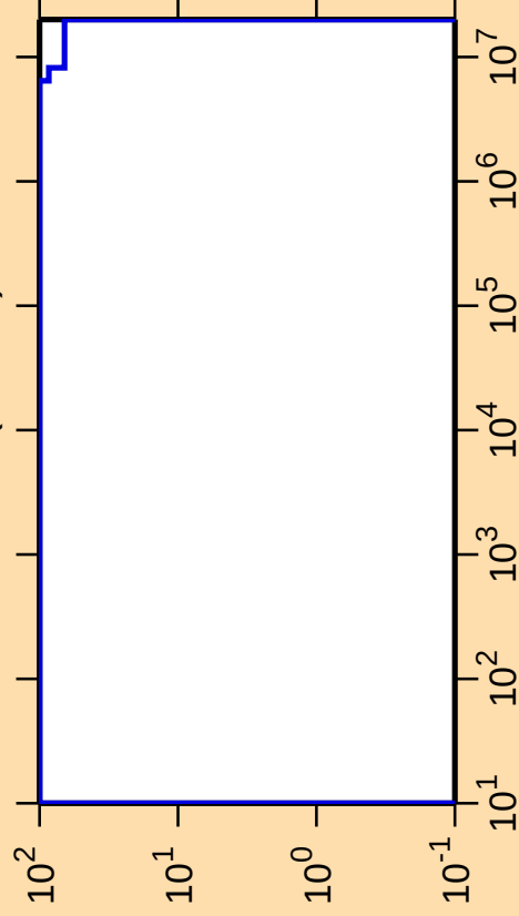
\Delta\sigma/\sigma vs. E for ^{127}\text{Ce}(n,\text{inel.})
