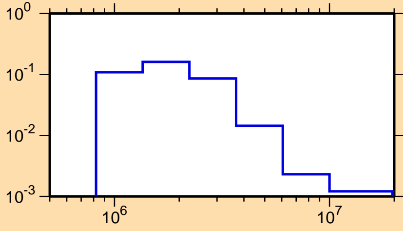
\sigma vs. E for ^{128}\text{Ce}(n,n_3)
