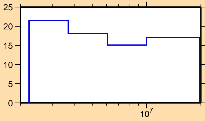
\Delta\sigma/\sigma vs. E for ^{128}\text{Ce}(n,n\text{onel.})
