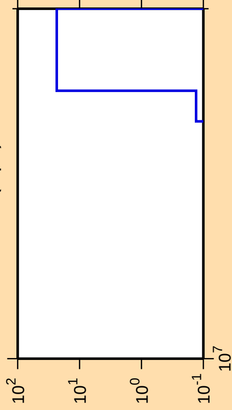
\Delta\sigma/\sigma vs. E for ^{137}\text{Ce}(n,\text{pd})
