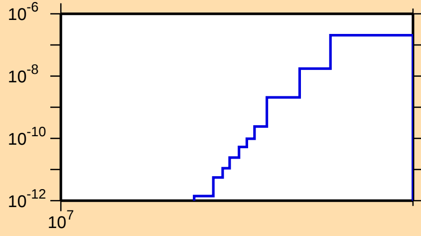
\sigma vs. E for ^{137}\text{Ce}(n,\text{He3})
