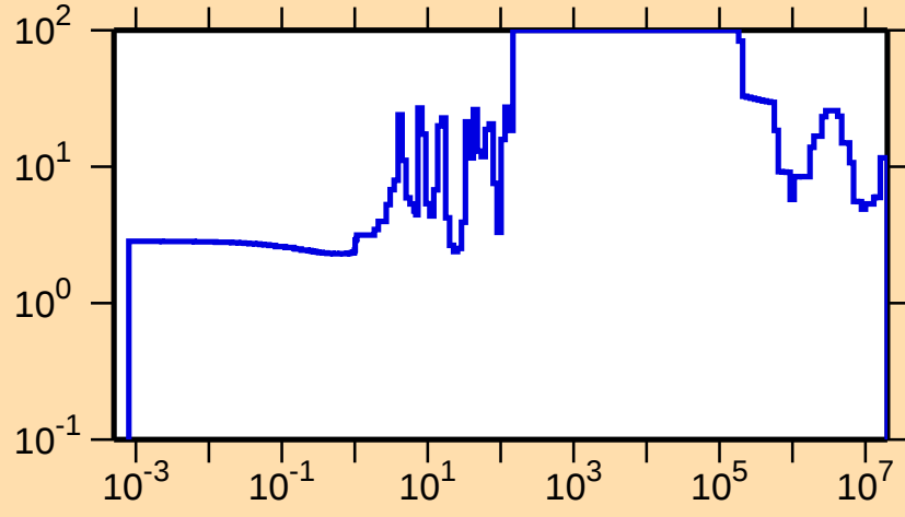
\Delta\sigma/\sigma vs. E for ^{137}\text{Ce}(n,\text{el.})
