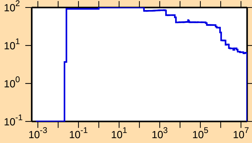
\Delta\sigma/\sigma vs. E for ^{137}\text{Ce}(n,\text{nonel.})
