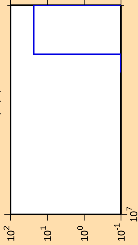
\Delta\sigma/\sigma vs. E for ^{137}\text{Ce}(n,\text{pt})
