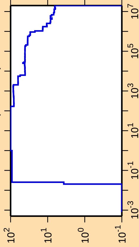
\Delta\sigma/\sigma vs. E for ^{137}\text{Ce}(n,\text{nonel.})
