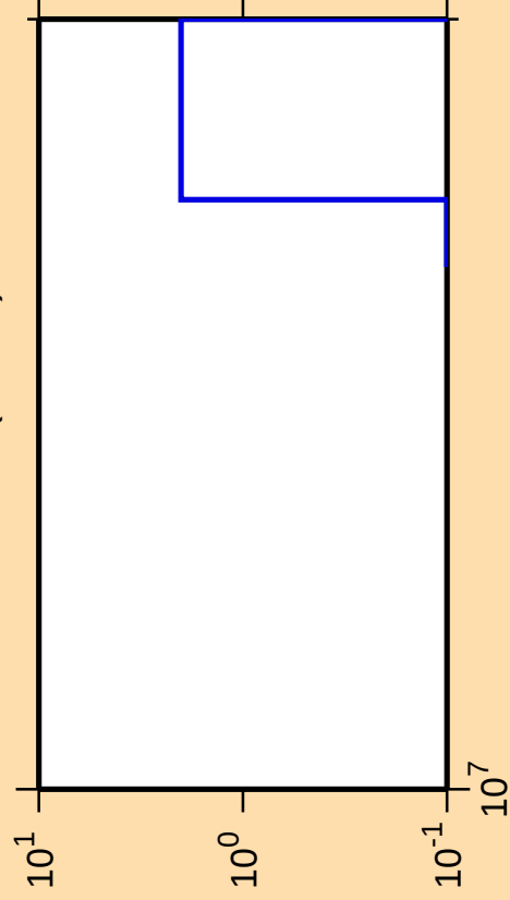
\Delta\sigma/\sigma vs. E for ^{137}\text{Ce} (mt 34)
