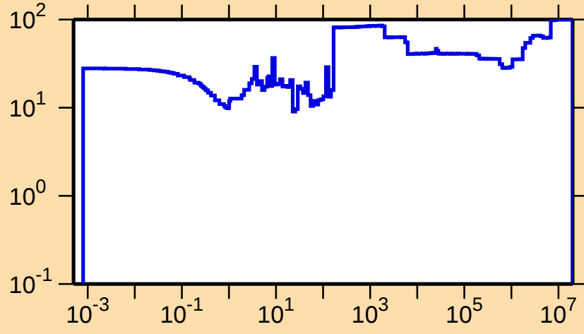
\Delta\sigma/\sigma vs. E for ^{137}\text{Ce}(n,\gamma)
