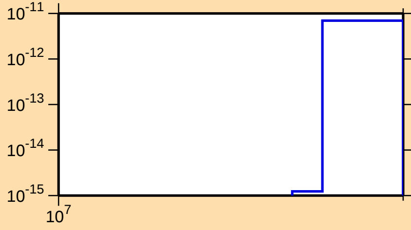
\sigma vs. E for ^{137}\text{Ce}(n,\text{pt})
