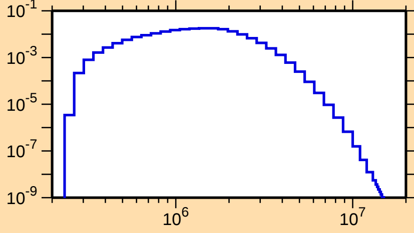
\sigma vs. E for ^{137}\text{Ce}(n,n_4)
