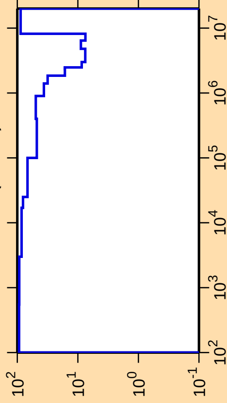
\Delta\sigma/\sigma vs. E for ^{137}\text{Ce}(n,\text{inel.})
