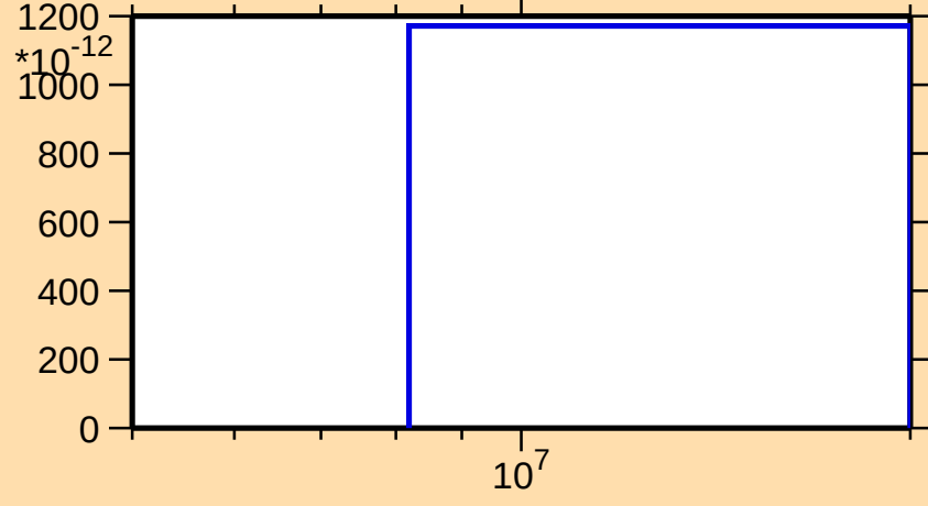
\sigma vs. E for ^{137}\text{Ce}(n,p\alpha)
