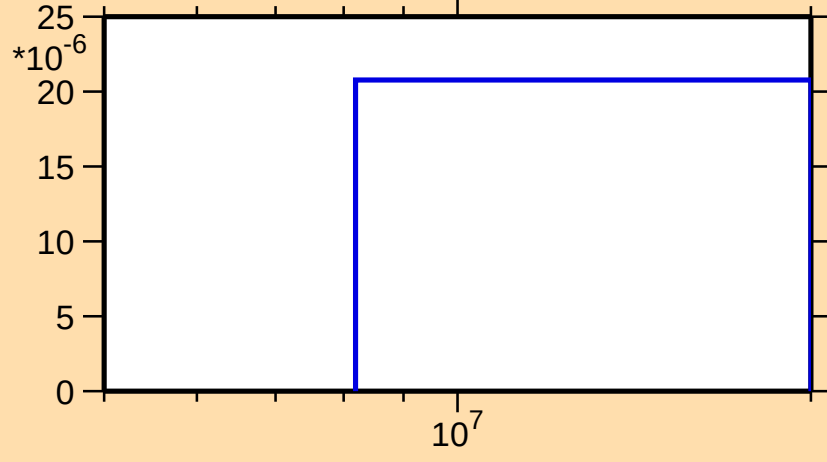
\sigma vs. E for ^{137}\text{Ce}(n,3n)
