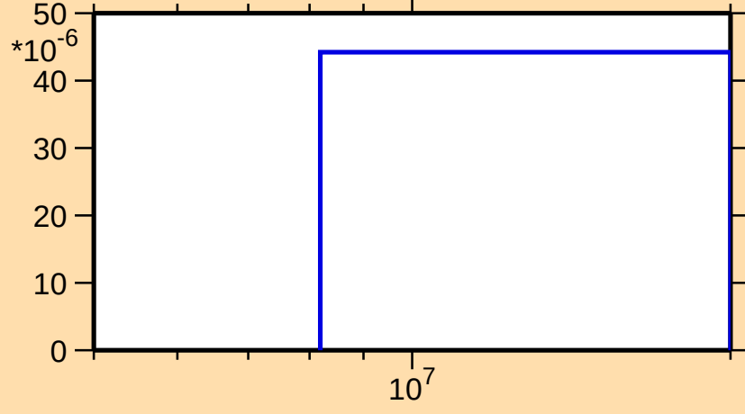
\sigma vs. E for ^{137}\text{Ce}(n,t)
