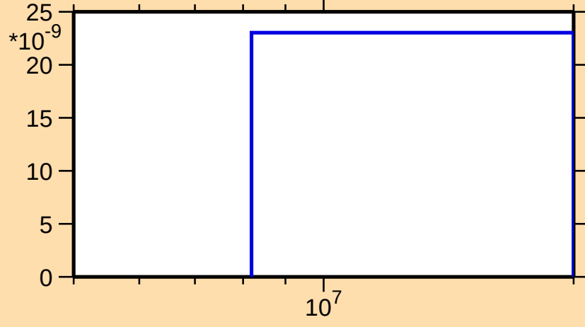
\sigma vs. E for ^{137}\text{Ce}(n,\text{nd})
