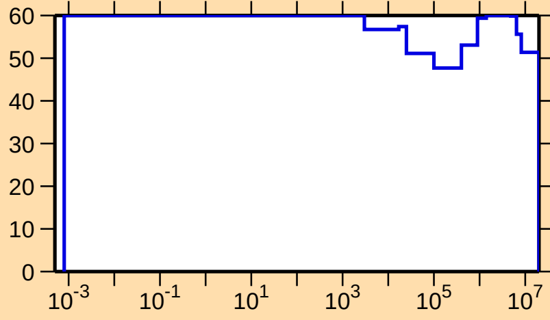
\Delta\sigma/\sigma vs. E for ^{137}\text{Ce}(n,p)
