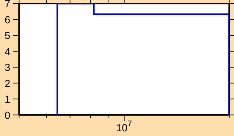
\Delta\sigma/\sigma vs. E for ^{137}\text{Ce}(n,\text{nonel.})
