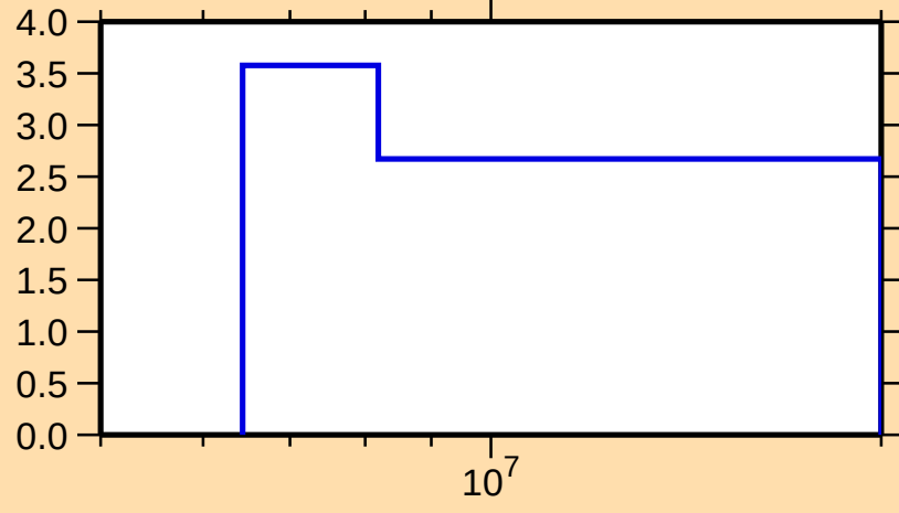
\Delta\sigma/\sigma vs. E for ^{137}\text{Ce}(n,\text{tot.})
