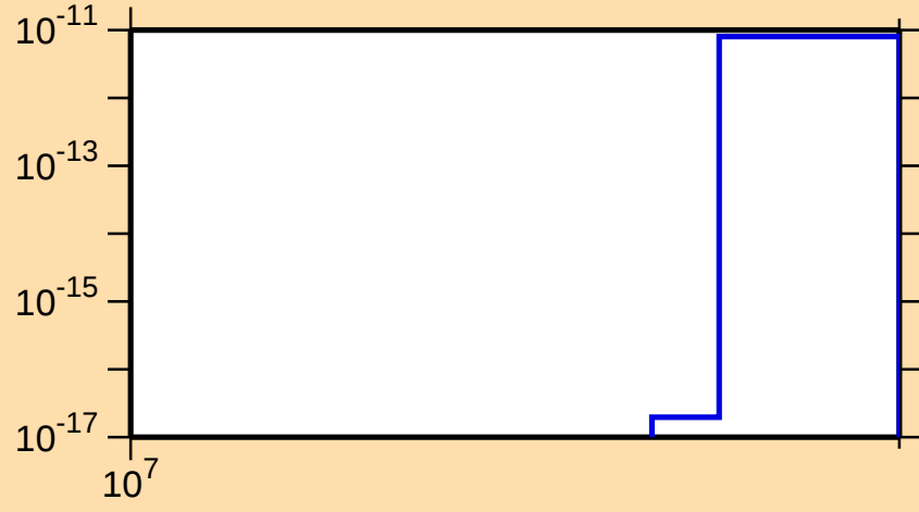
\sigma vs. E for ^{138}\text{Ce}(n,\text{nt})
