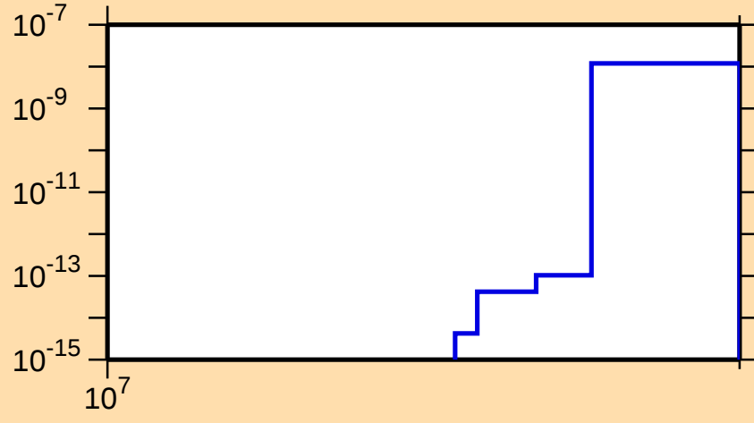
\sigma vs. E for ^{138}\text{Ce}(n,\text{nd})
