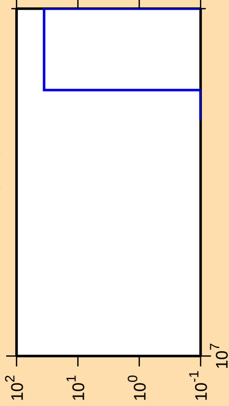
\Delta\sigma/\sigma vs. E for ^{138}\text{Ce}(n,\text{nt})
