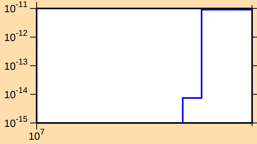
\sigma vs. E for ^{138}\text{Ce}(n,\text{pd})
