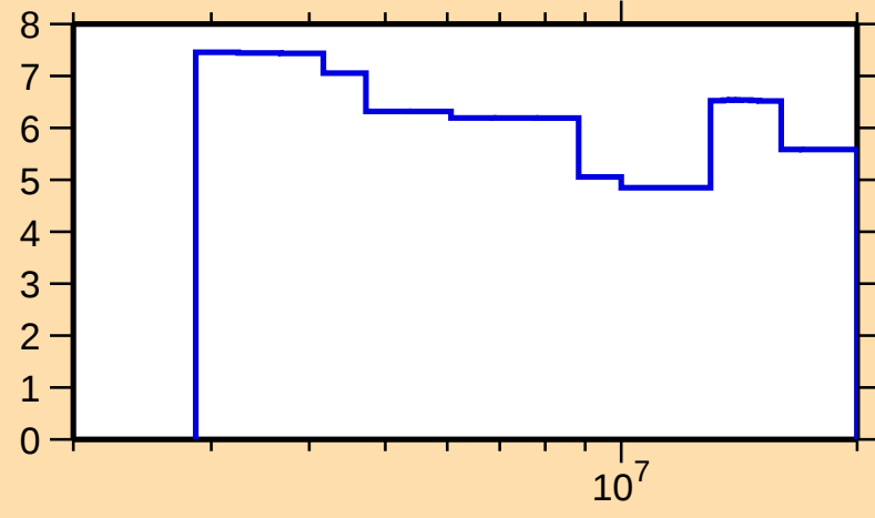
\Delta\sigma/\sigma vs. E for ^{138}\text{Ce}(n,n\text{onel.})
