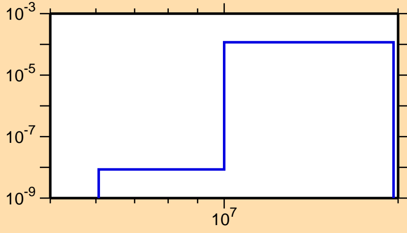
\sigma vs. E for ^{138}\text{Ce}(n,n\alpha)
