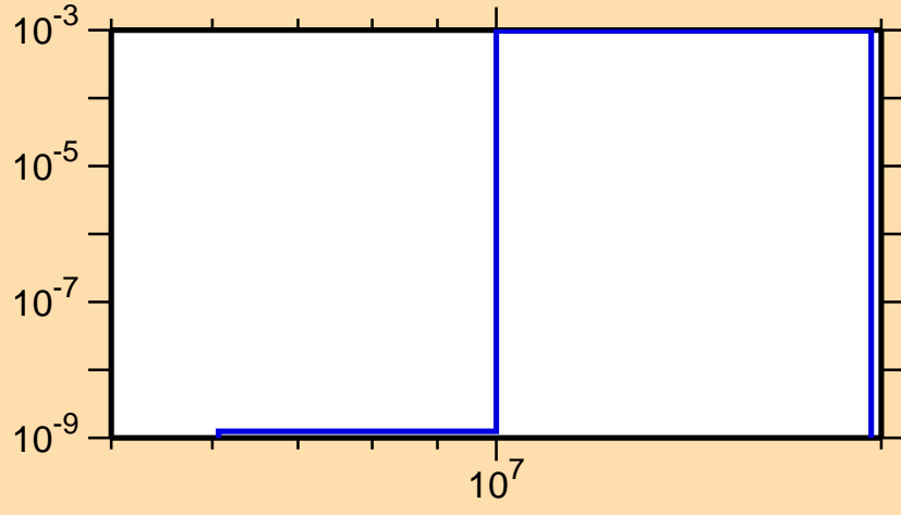
\sigma vs. E for ^{138}\text{Ce}(n,d)
