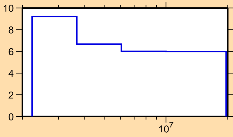
\Delta\sigma/\sigma vs. E for ^{138}\text{Ce}(n,n\text{onel.})
