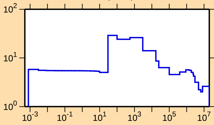
\sigma vs. E for ^{138}\text{Ce}(n,\text{el.})
