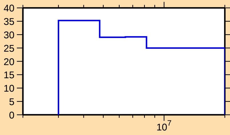
\Delta\sigma/\sigma vs. E for ^{138}\text{Ce}(n,n_1)
