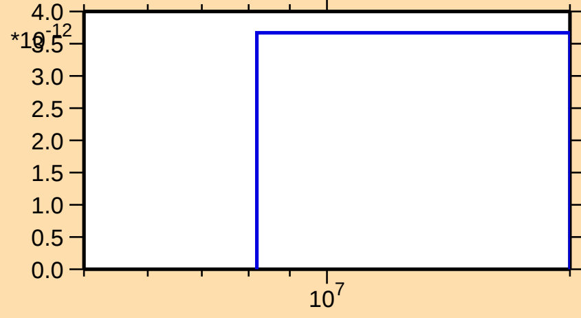
\sigma vs. E for ^{138}\text{Ce}(n,2n\alpha)
