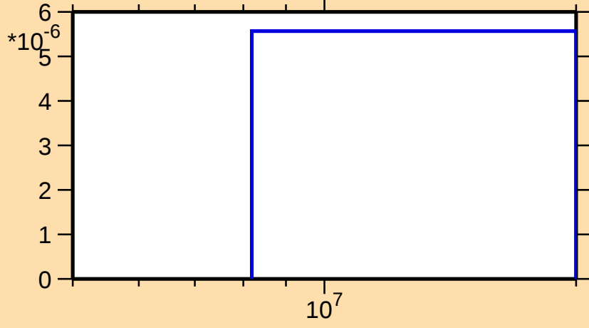
\sigma vs. E for ^{138}\text{Ce}(n,t)
