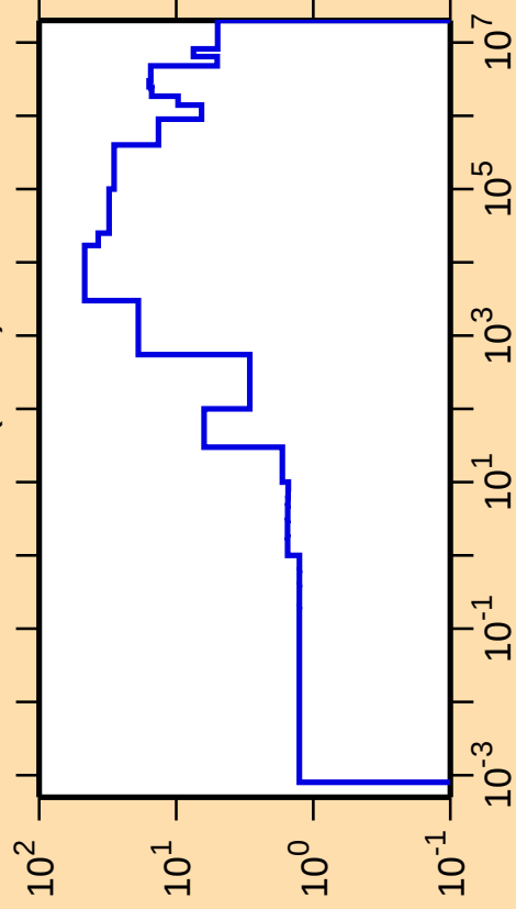
\Delta\sigma/\sigma vs. E for ^{138}\text{Ce}(n,\text{el.})
