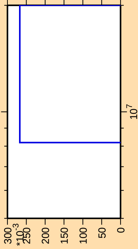
\Delta\sigma/\sigma vs. E for ^{138}\text{Ce}(n,\text{pd})
