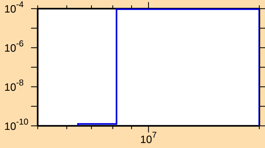
\sigma vs. E for ^{138}\text{Ce}(n,n\alpha)
