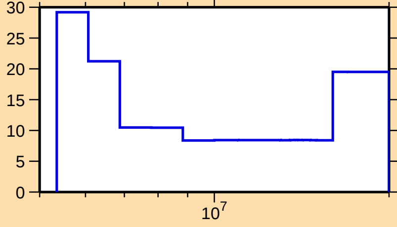
\Delta\sigma/\sigma vs. E for ^{141}\text{Ce}(n,2n)
