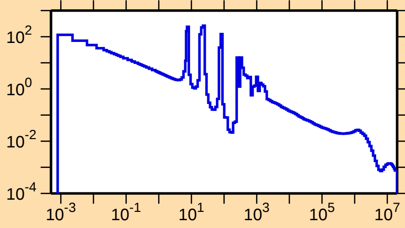
\sigma vs. E for ^{141}\text{Ce}(n,\gamma)
