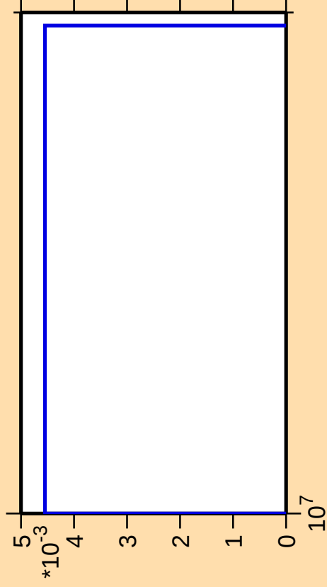
\Delta\sigma/\sigma vs. E for ^{141}\text{Ce} (mt 34)
