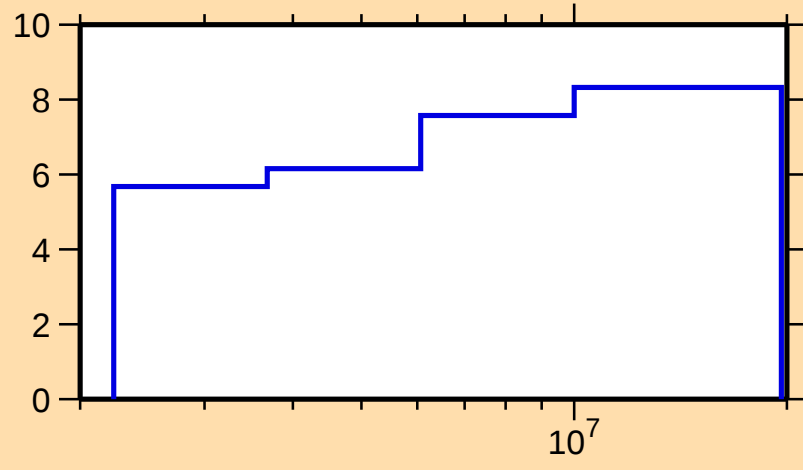
\Delta\sigma/\sigma vs. E for ^{141}\text{Ce}(n,n\text{onel.})
