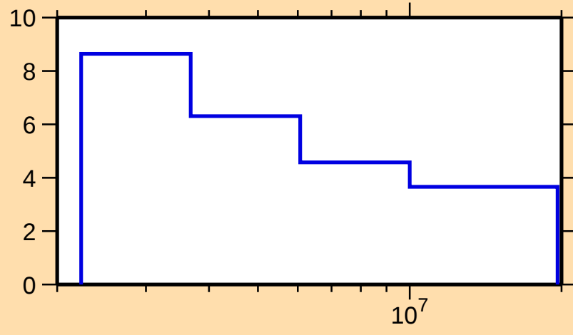
\Delta\sigma/\sigma vs. E for ^{141}\text{Ce}(n,\text{tot.})
