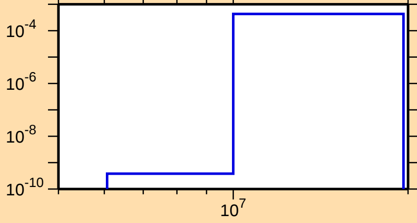
\sigma vs. E for ^{141}\text{Ce}(n,t)
