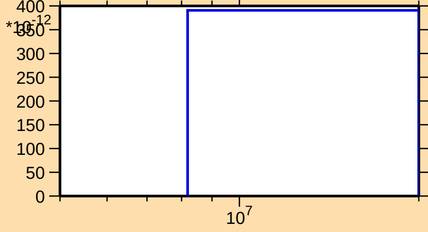
\sigma vs. E for ^{141}\text{Ce}(n,\text{nt})
