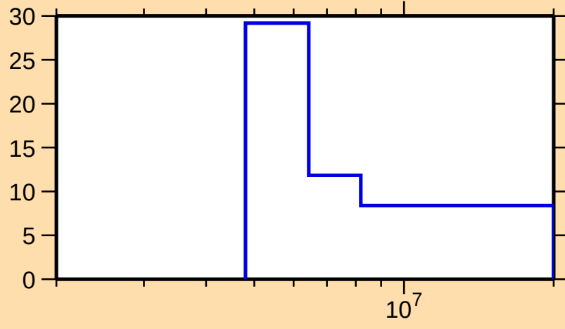
\Delta\sigma/\sigma vs. E for ^{141}\text{Ce}(n,2n)
