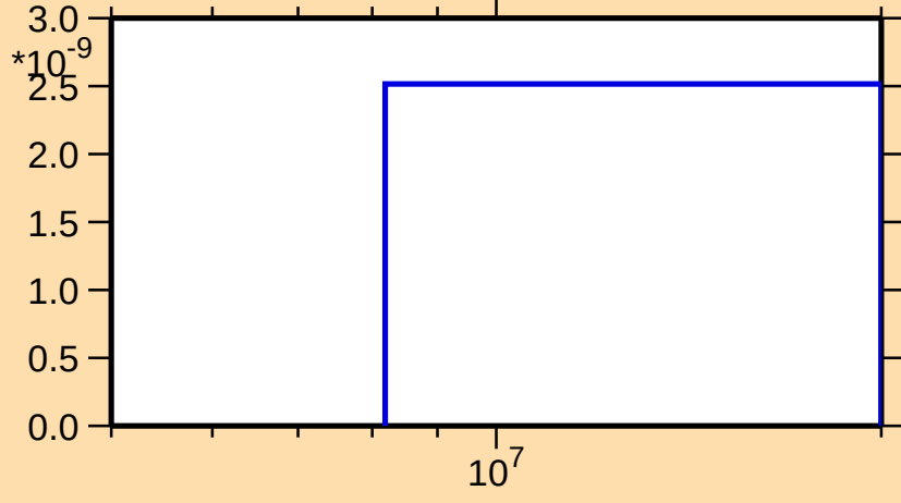
\sigma vs. E for ^{141}\text{Ce}(n,2n\alpha)
