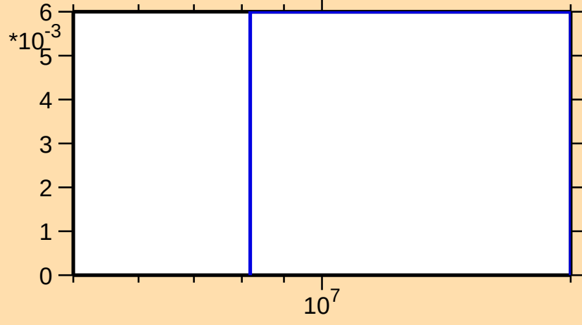
\sigma vs. E for ^{141}\text{Ce}(n,3n)
