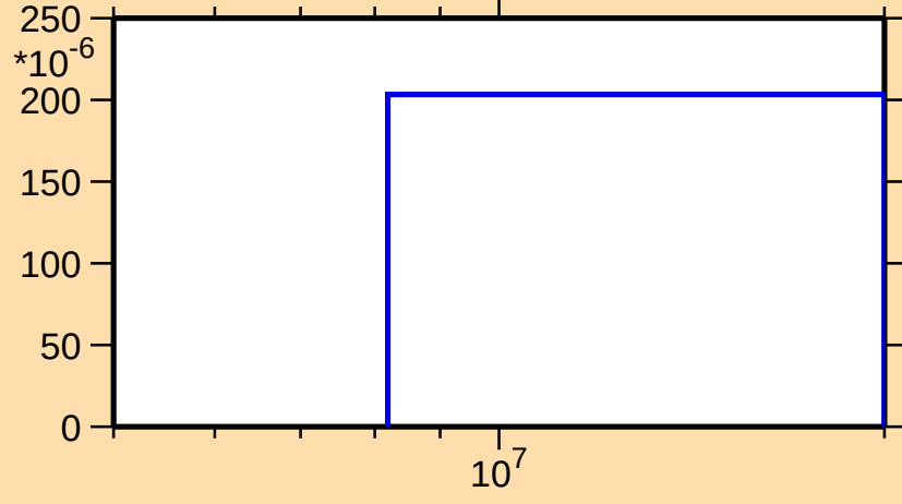
\sigma vs. E for ^{141}\text{Ce}(n,np)
