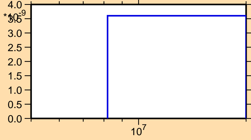
\sigma vs. E for ^{143}\text{Ce}(n,2np)
