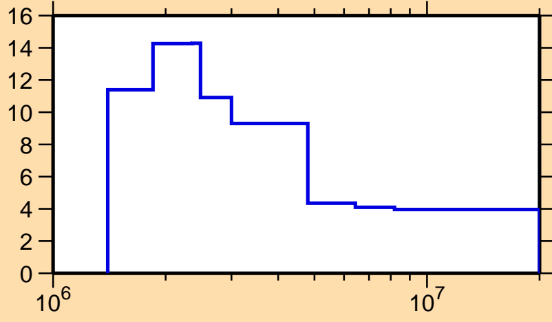
\Delta\sigma/\sigma vs. E for ^{143}\text{Ce}(n,\text{tot.})
