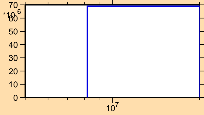
\sigma vs. E for ^{143}\text{Ce}(n,t)
