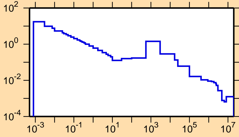
\sigma vs. E for ^{143}\text{Ce}(n,\gamma)
