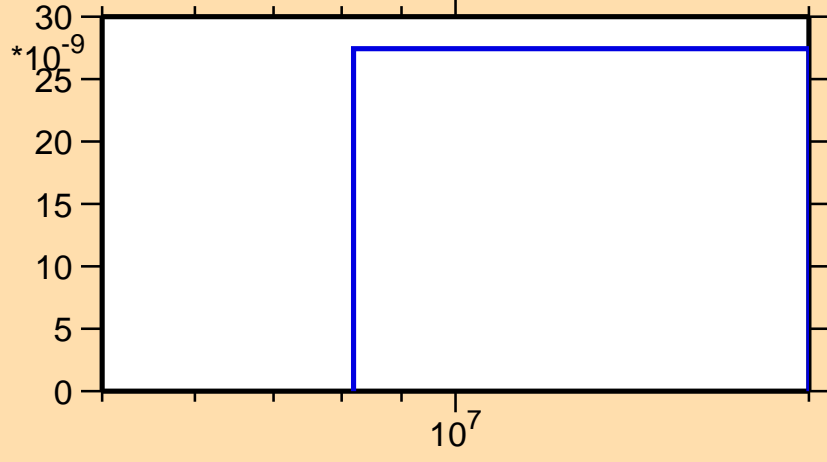
\sigma vs. E for ^{143}\text{Ce}(n,nt)
