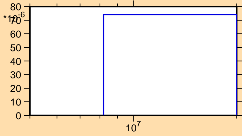
\sigma vs. E for ^{143}\text{Ce}(n,np)
