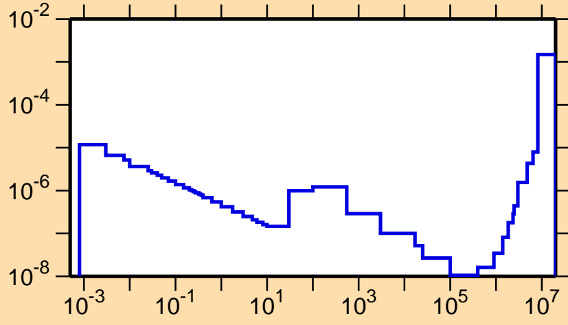
\sigma vs. E for ^{143}\text{Ce}(n,\alpha)
