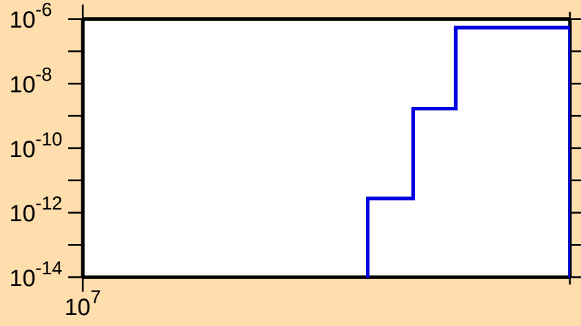
\sigma vs. E for ^{149}\text{Ce}(n,\text{nd})
