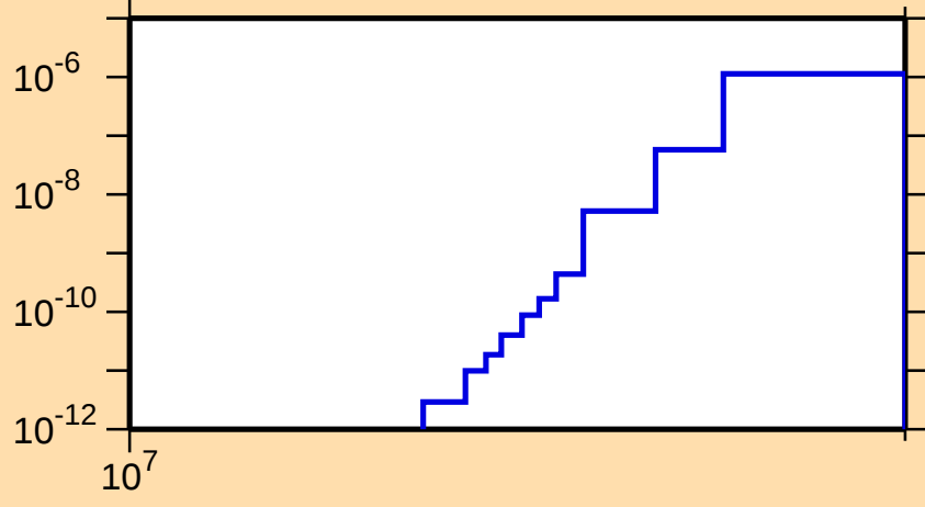
\sigma vs. E for ^{149}\text{Ce}(n,2n\alpha)
