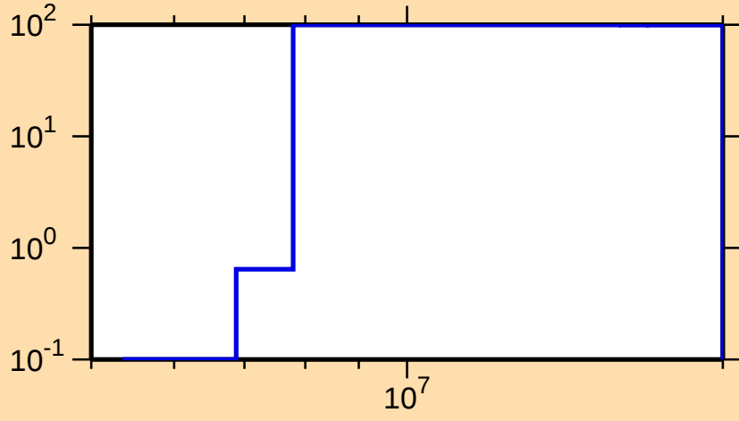
\Delta\sigma/\sigma vs. E for ^{149}\text{Ce}(n,p)
