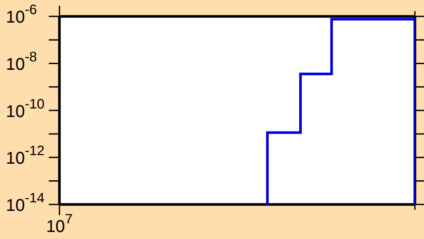
\sigma vs. E for ^{149}\text{Ce}(n,\text{nt})
