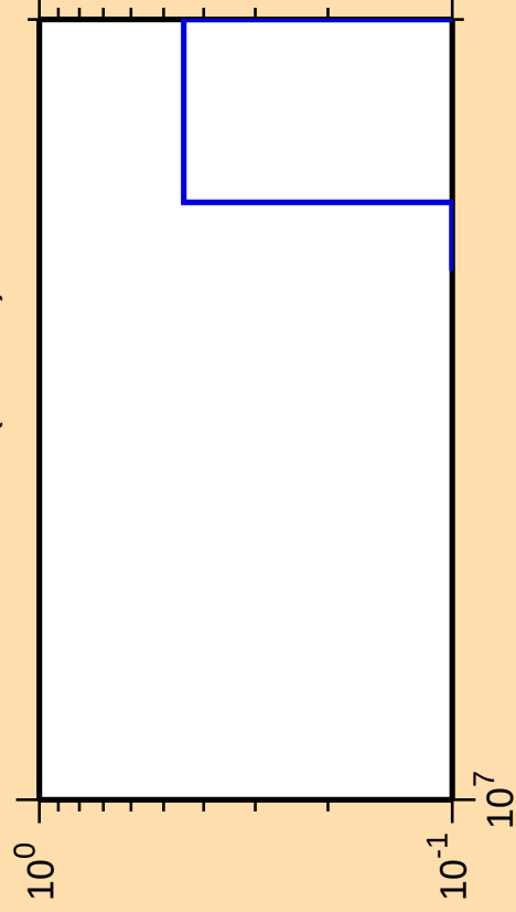
\Delta\sigma/\sigma vs. E for ^{149}\text{Ce}(n,3n\alpha)
