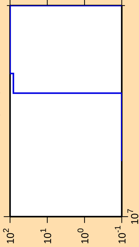
\Delta\sigma/\sigma vs. E for ^{149}\text{Ce}(n,\text{nt})
