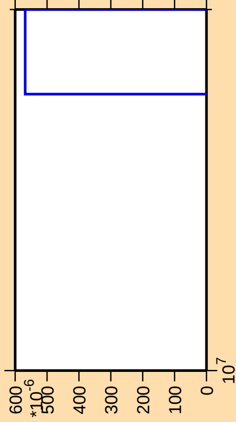
\Delta\sigma/\sigma vs. E for ^{149}\text{Ce}(\text{mt 11})
