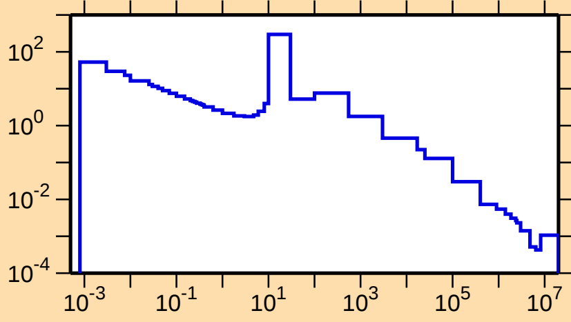
\sigma vs. E for ^{149}\text{Ce}(n,\gamma)
