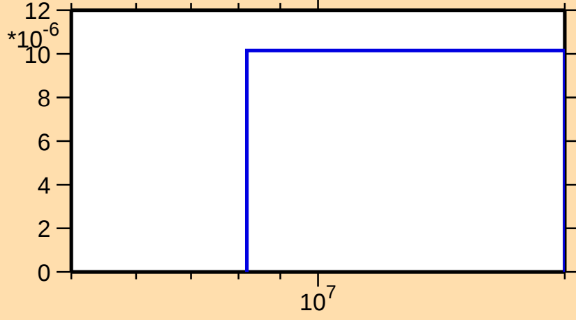
\sigma vs. E for ^{149}\text{Ce}(n,t)
