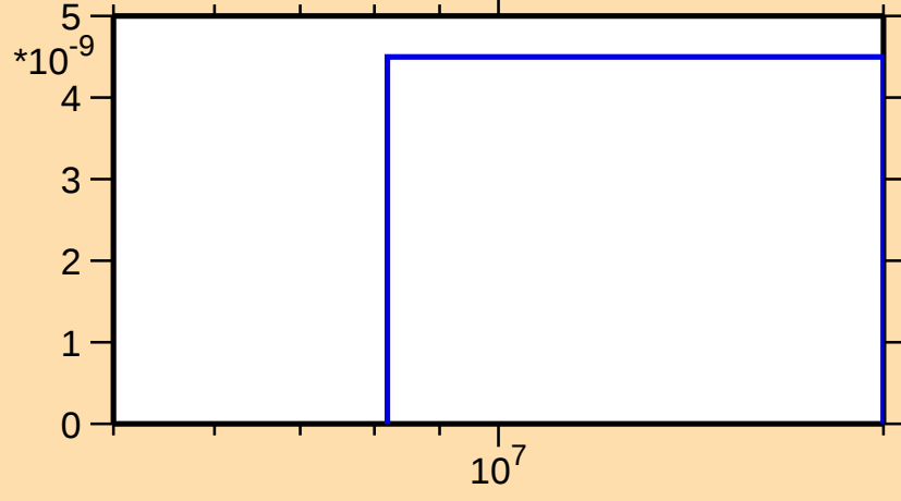
\sigma vs. E for ^{149}\text{Ce}(n,\text{nd})
