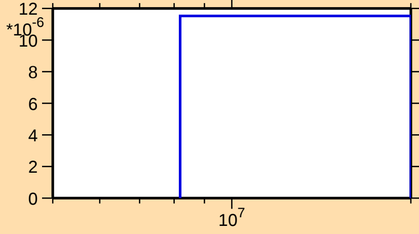
\sigma vs. E for ^{149}\text{Ce}(n,d)
