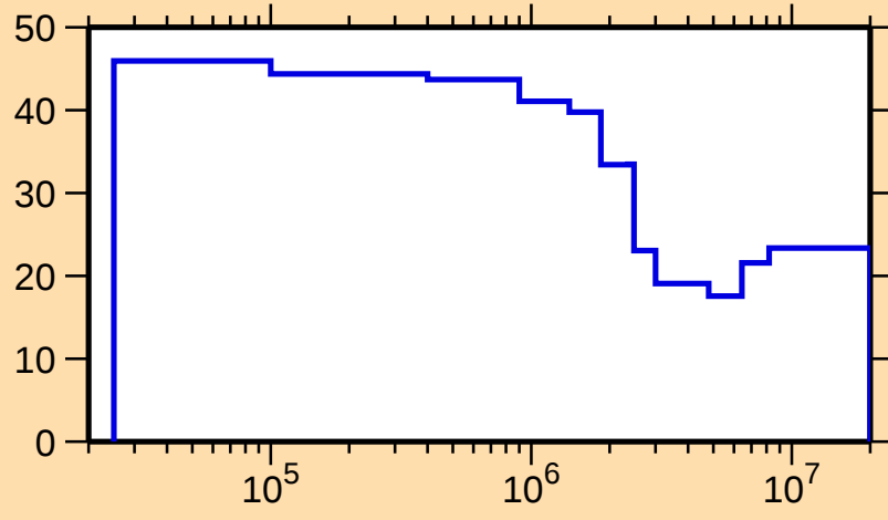
\Delta\sigma/\sigma vs. E for ^{149}\text{Ce}(n,\text{nonel.})
