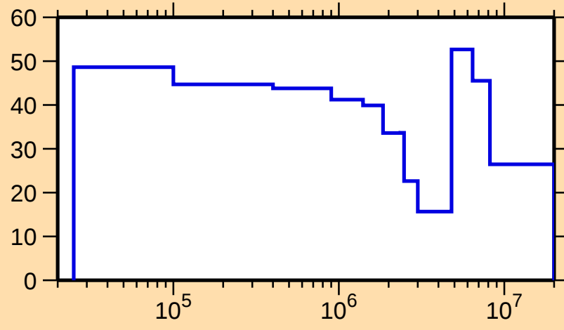
\Delta\sigma/\sigma vs. E for ^{149}\text{Ce}(n,\text{inel.})
