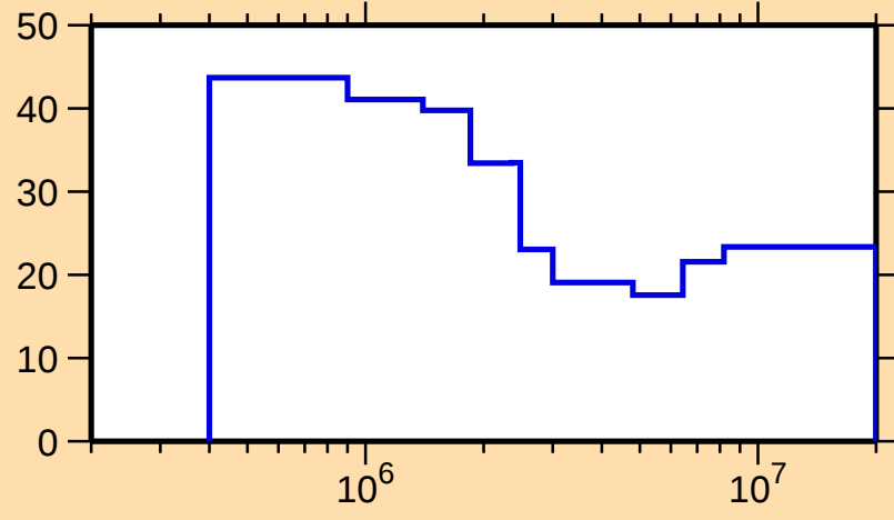
\Delta\sigma/\sigma vs. E for ^{149}\text{Ce}(n,n\text{onel.})
