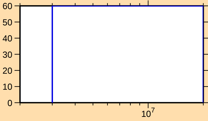
\Delta\sigma/\sigma vs. E for ^{149}\text{Ce}(n,\text{el.})
