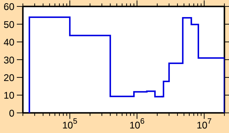
\Delta\sigma/\sigma vs. E for ^{149}\text{Ce}(n,\text{tot.})
