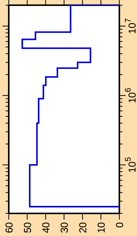
\Delta\sigma/\sigma vs. E for ^{149}\text{Ce}(n,\text{inel.})
