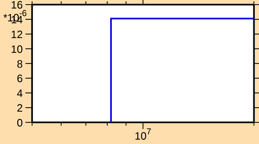
\sigma vs. E for ^{149}\text{Ce}(n,n\alpha)
