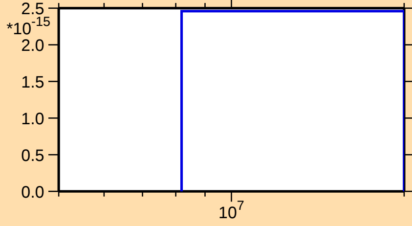
\sigma vs. E for ^{149}\text{Ce}(n,3n\alpha)
