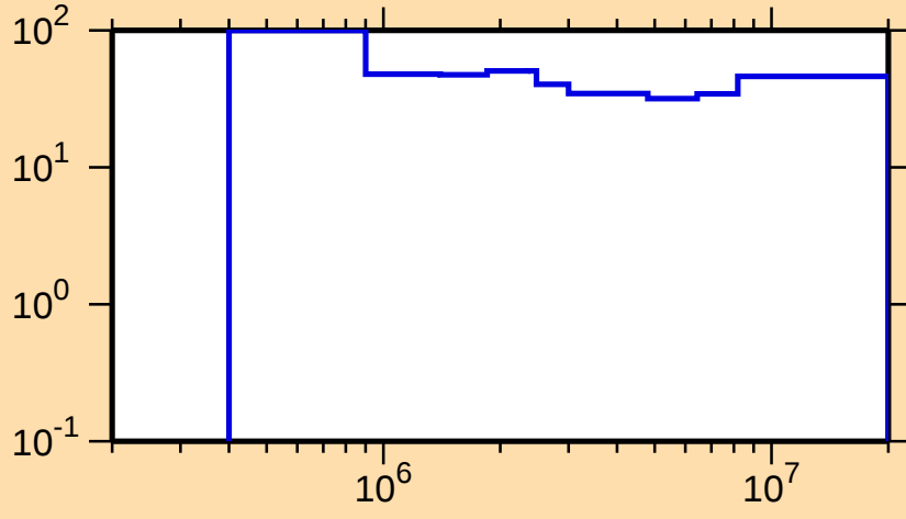
\Delta\sigma/\sigma vs. E for ^{149}\text{Ce}(n,n\text{cont.})
