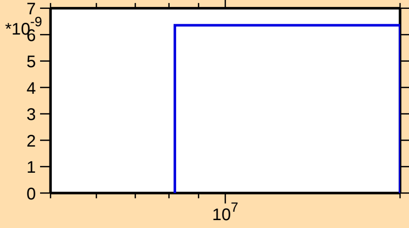
\sigma vs. E for ^{149}\text{Ce}(n,nt)
