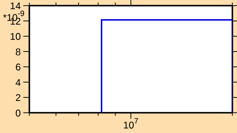
\sigma vs. E for ^{149}\text{Ce}(n,2n\alpha)
