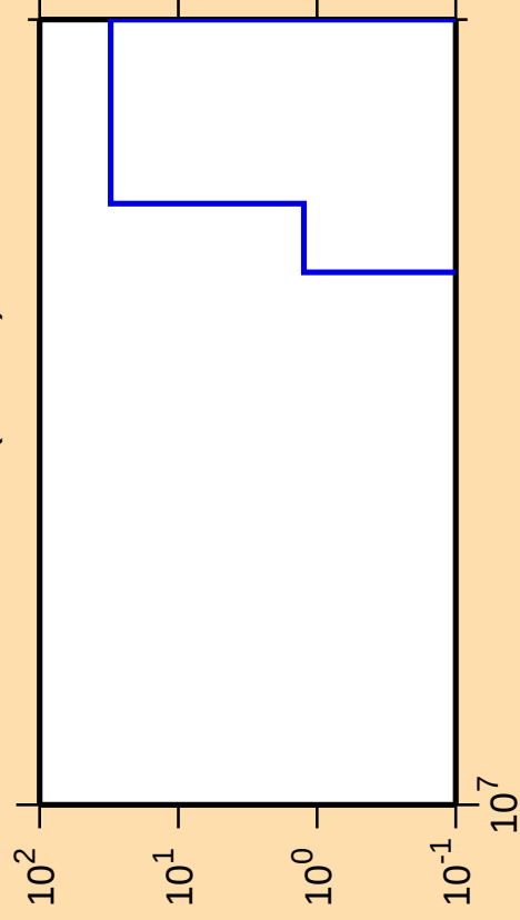
\Delta\sigma/\sigma vs. E for ^{241}\text{Cf}(\text{mt } 34)
