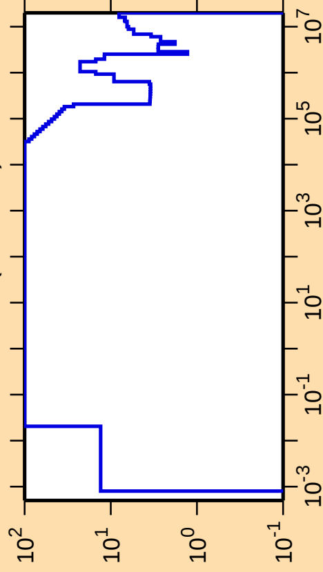
\Delta\sigma/\sigma vs. E for ^{241}\text{Cf}(n,\text{nonel.})
