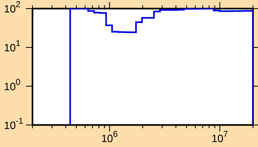
\Delta\sigma/\sigma vs. E for ^{241}\text{Cf}(n,n\text{cont.})
