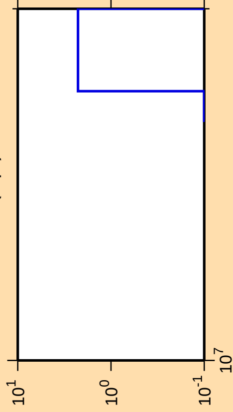
\Delta\sigma/\sigma vs. E for ^{241}\text{Cf}(n,pt)
