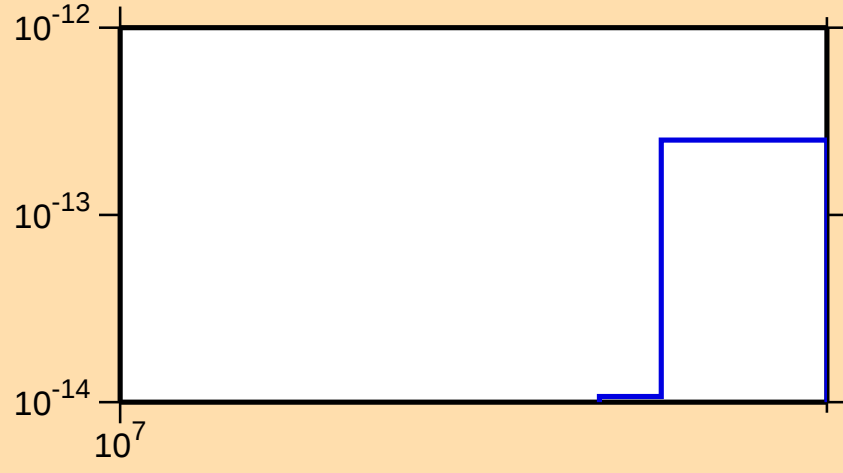
\sigma vs. E for ^{241}\text{Cf}(n,pt)
