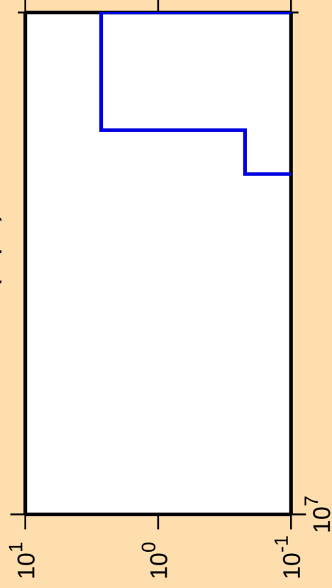
\Delta\sigma/\sigma vs. E for ^{241}\text{Cf}(n,\text{pd})
