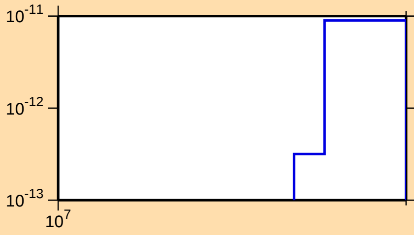
\sigma vs. E for ^{241}\text{Cf}(n,3n\alpha)
