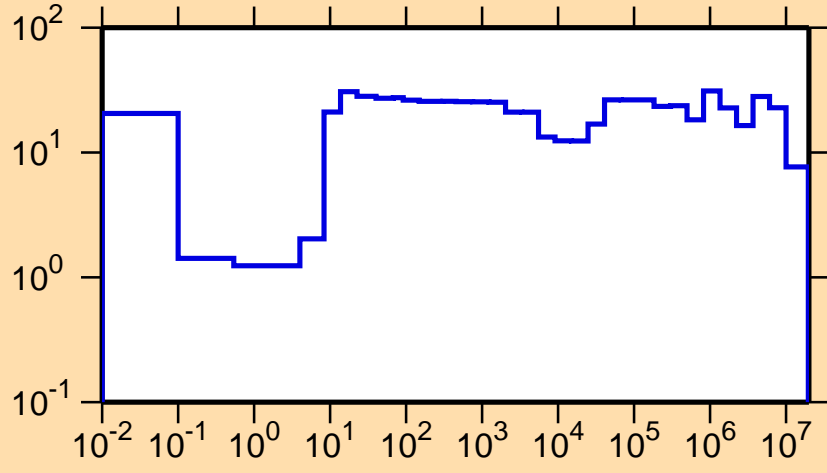
\Delta\sigma/\sigma vs. E for ^{241}\text{Cf}(n,el.)
