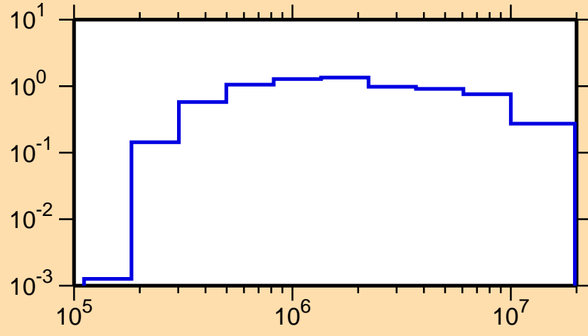
\sigma vs. E for ^{241}\text{Cf}(n,\text{inel.})
