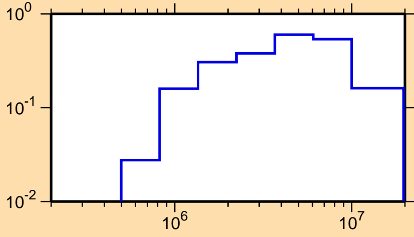
\sigma vs. E for ^{241}\text{Cf}(n,n\text{cont.})
