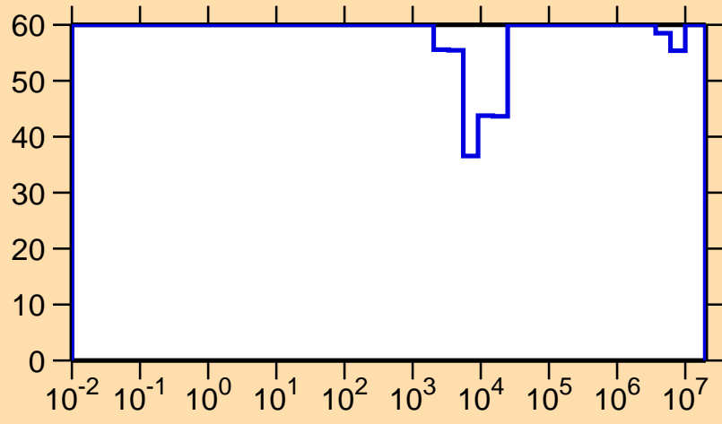
\Delta\sigma/\sigma vs. E for ^{241}\text{Cf}(n,p)
