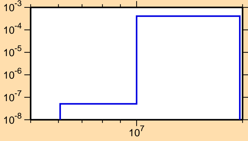
\sigma vs. E for ^{241}\text{Cf}(n,np)
