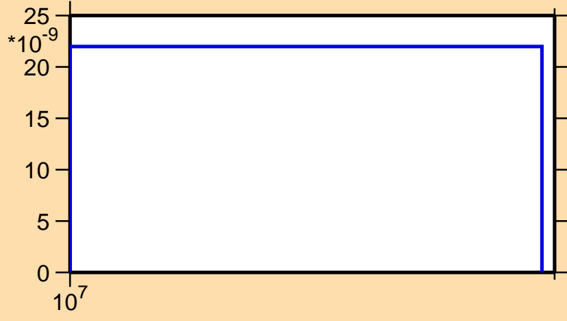
\sigma vs. E for ^{241}\text{Cf}(n,nd)
