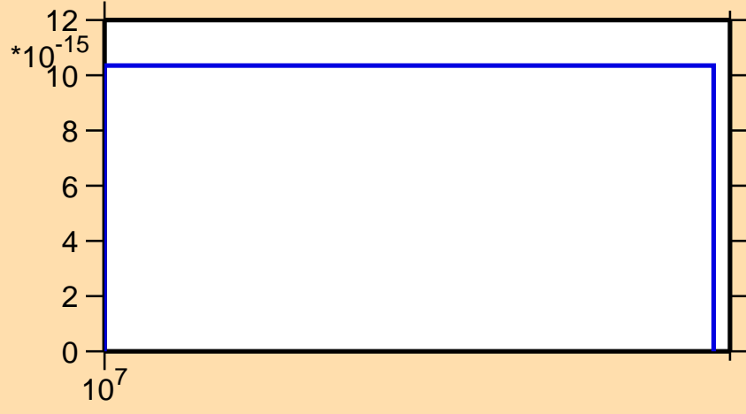
\sigma vs. E for ^{241}\text{Cf}(n,pd)
