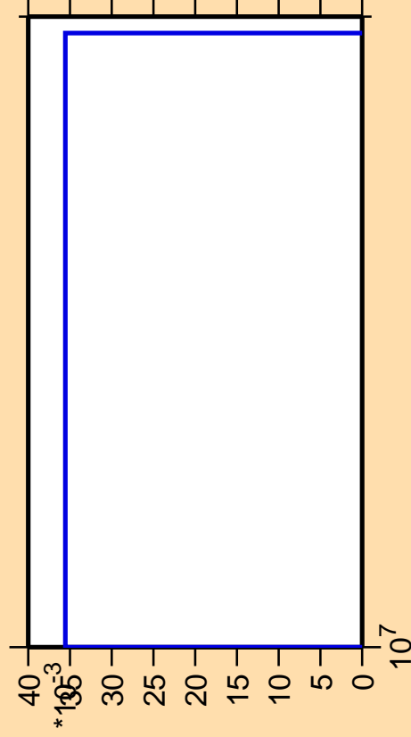
\Delta\sigma/\sigma vs. E for ^{241}\text{Cf}(n,pd)
