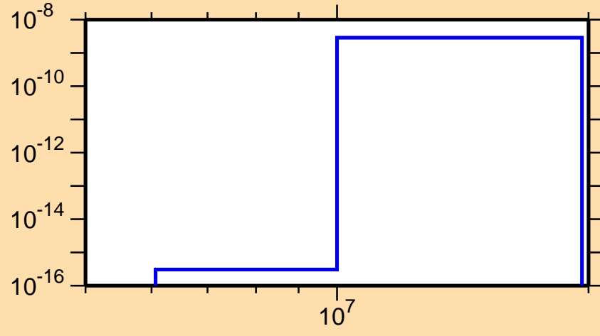
\sigma vs. E for ^{241}\text{Cf}(n,\text{He3})
