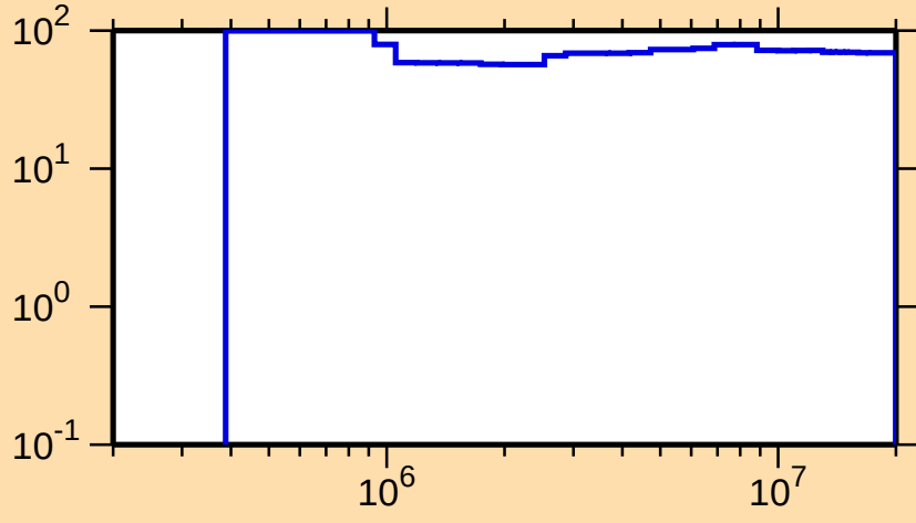
\Delta\sigma/\sigma vs. E for ^{243}\text{Cf}(n,n\text{cont.})
