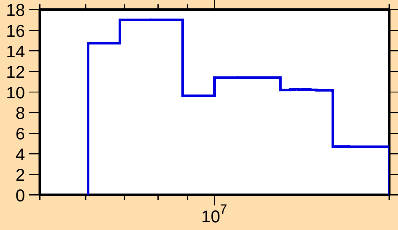
\Delta\sigma/\sigma vs. E for ^{243}\text{Cf}(n,\text{el.})
