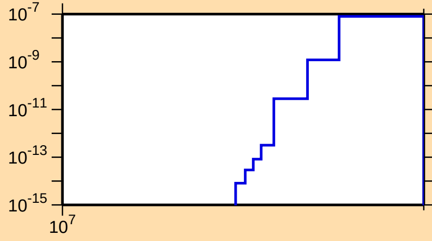
\sigma vs. E for ^{243}\text{Cf}(n,nt)
