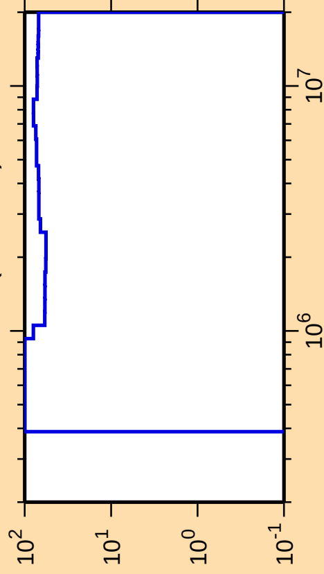
\Delta\sigma/\sigma vs. E for ^{243}\text{Cf}(n,\text{ncont.})
