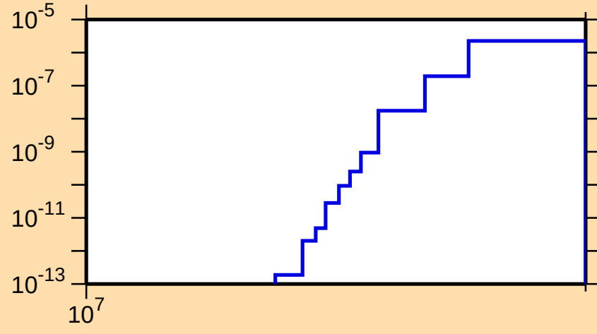
\sigma vs. E for ^{243}\text{Cf}(n,2np)
