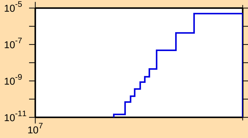
\sigma vs. E for ^{243}\text{Cf}(n,nd)
