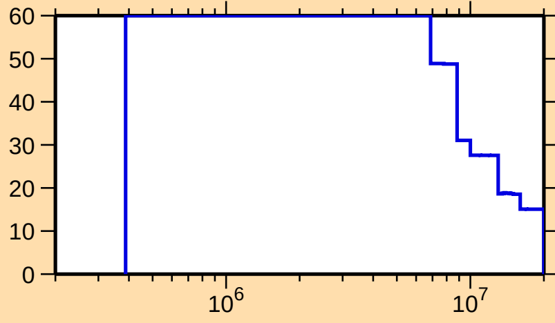
\Delta\sigma/\sigma vs. E for ^{243}\text{Cf}(n,f)
