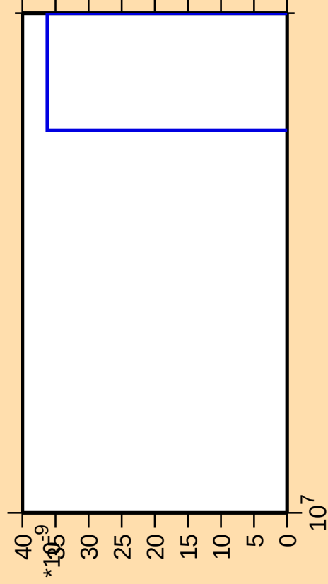
\Delta\sigma/\sigma vs. E for ^{243}\text{Cf}(\text{mt } 42)
