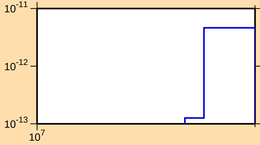
\sigma vs. E for ^{243}\text{Cf}(\text{mt } 34)
