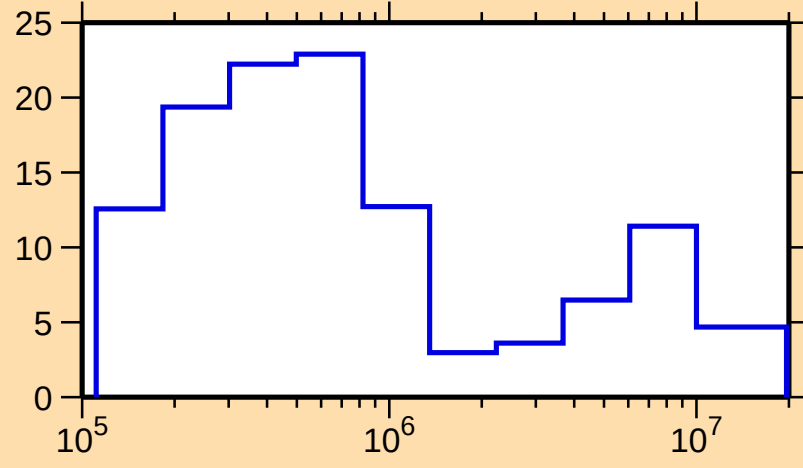
\Delta\sigma/\sigma vs. E for ^{243}\text{Cf}(n,\text{tot.})
