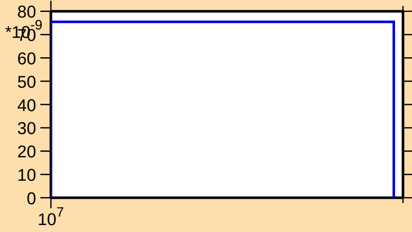
\sigma vs. E for ^{243}\text{Cf}(n,\text{nd})
