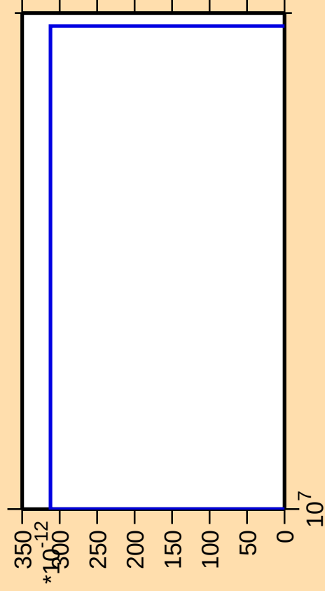
\Delta\sigma/\sigma vs. E for ^{243}\text{Cf}(\text{mt } 42)
