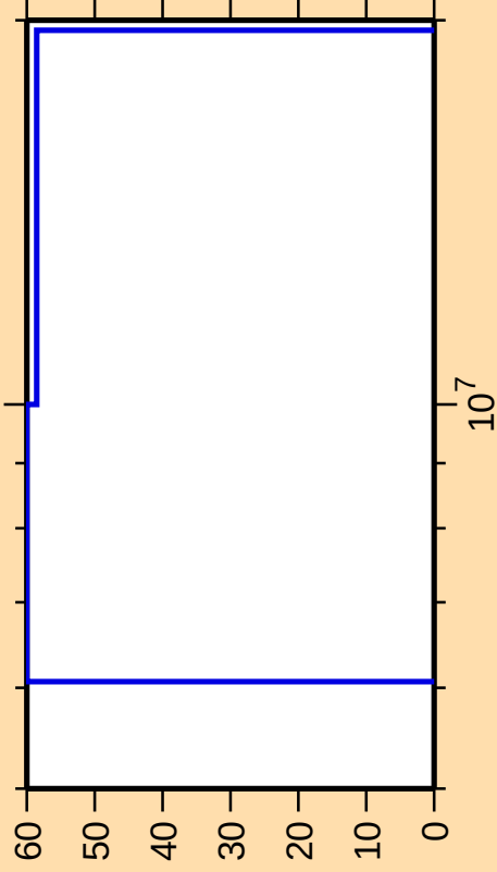
\Delta\sigma/\sigma vs. E for ^{243}\text{Cf}(n,d)
