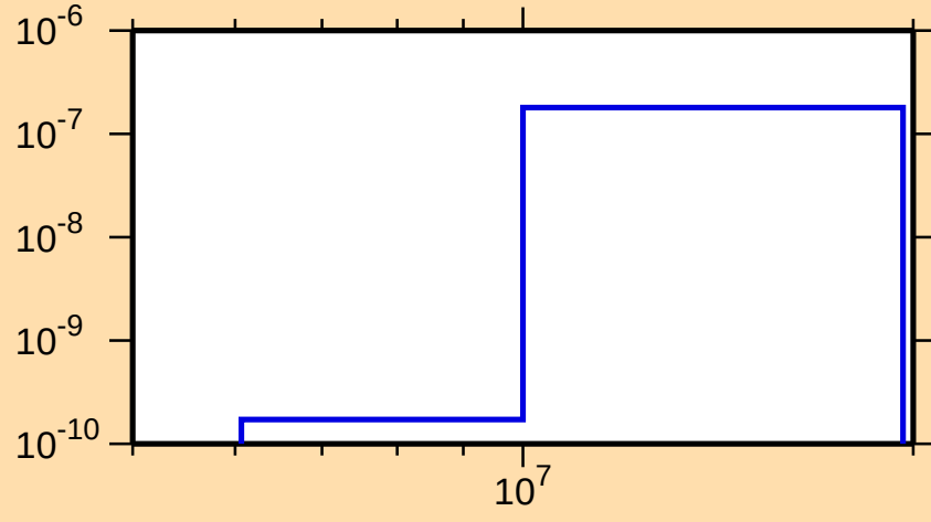
\sigma vs. E for ^{243}\text{Cf}(n,2n\alpha)
