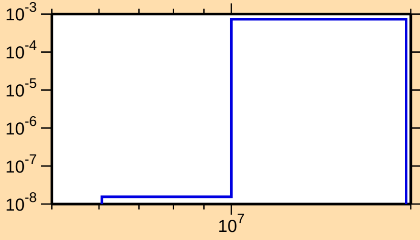
\sigma vs. E for ^{243}\text{Cf}(n,d)
