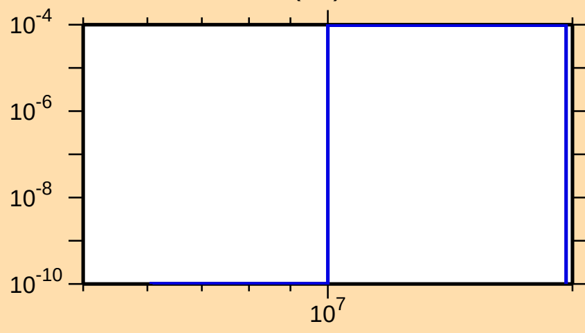
\sigma vs. E for ^{243}\text{Cf}(n,t)
