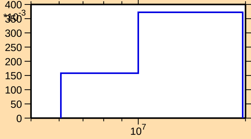
\sigma vs. E for ^{243}\text{Cf}(n,2n)
