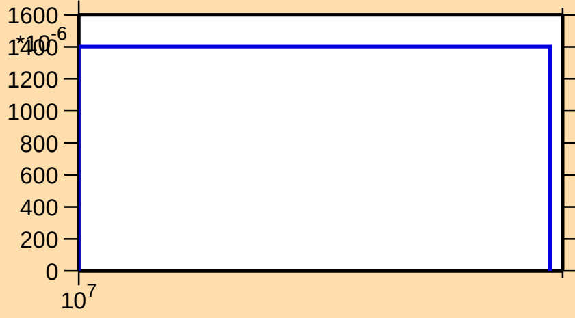
\sigma vs. E for ^{243}\text{Cf}(n,3n)
