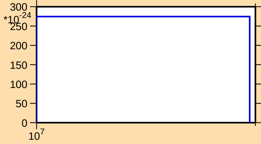
\sigma vs. E for ^{243}\text{Cf}(\text{mt } 42)
