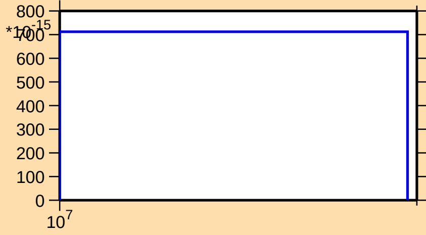
\sigma vs. E for ^{243}\text{Cf}(n,3n\alpha)
