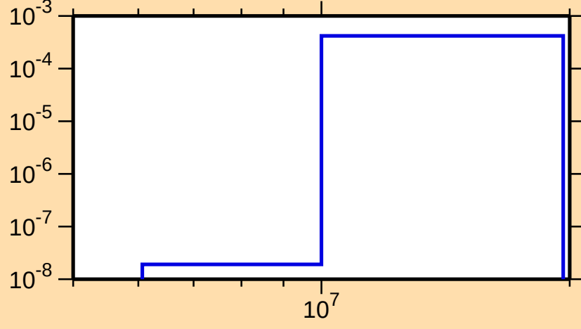
\sigma vs. E for ^{243}\text{Cf}(n,np)
