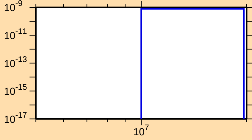
\sigma vs. E for ^{243}\text{Cf}(n,\text{He3})
