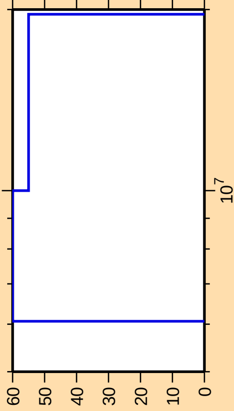
\Delta\sigma/\sigma vs. E for ^{243}\text{Cf}(n,t)
