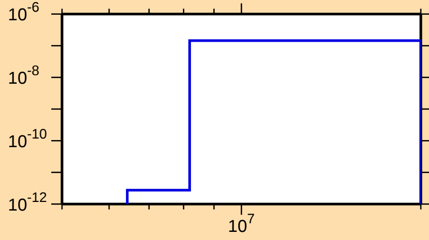
\sigma vs. E for ^{243}\text{Cf}(n,2n\alpha)
