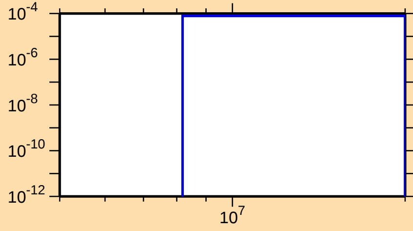
\sigma vs. E for ^{243}\text{Cf}(n,t)
