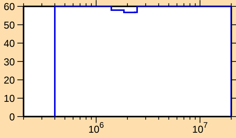
\Delta\sigma/\sigma vs. E for ^{243}\text{Cf}(n,n\text{cont.})
