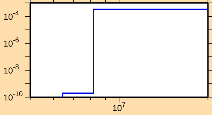
\sigma vs. E for ^{243}\text{Cf}(n,np)
