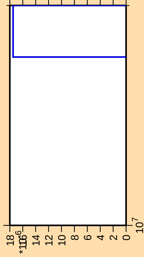
\Delta\sigma/\sigma vs. E for ^{246}\text{Cf}(\text{mt } 42)
