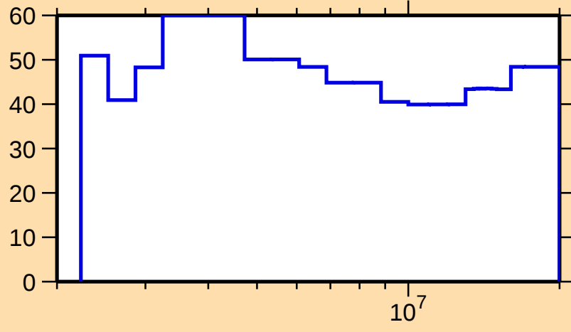
\Delta\sigma/\sigma vs. E for ^{246}\text{Cf}(n,n_1)
