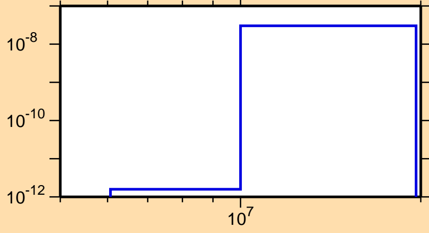
\sigma vs. E for ^{246}\text{Cf}(n,2n\alpha)
