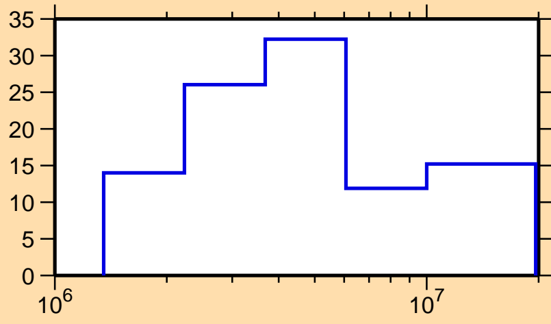
\Delta\sigma/\sigma vs. E for ^{246}\text{Cf}(n,el.)
