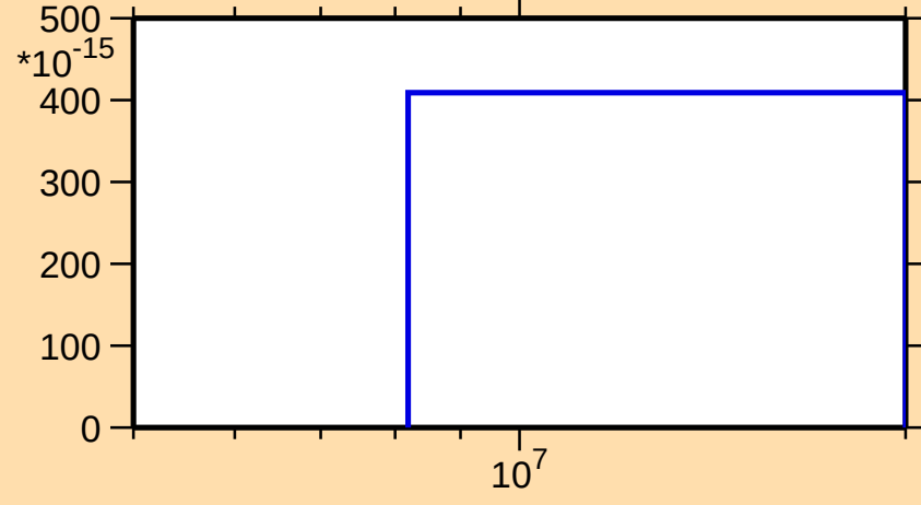
\sigma vs. E for ^{246}\text{Cf}(n,p\alpha)
