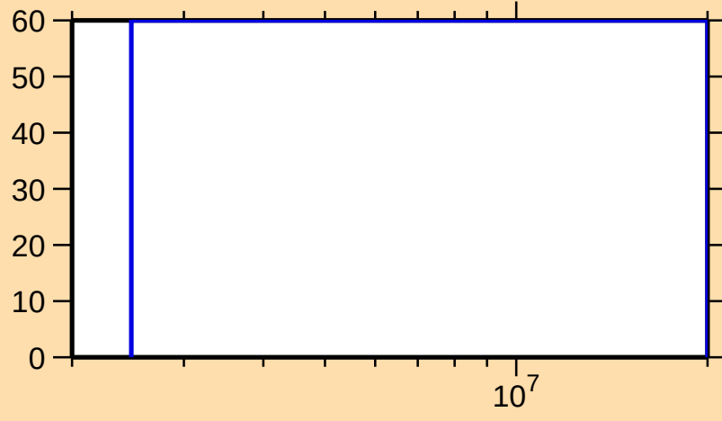
\Delta\sigma/\sigma vs. E for ^{246}\text{Cf}(n,f)
