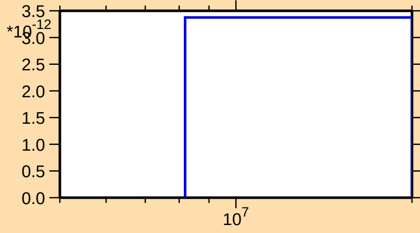
\sigma vs. E for ^{246}\text{Cf}(n,3n\alpha)
