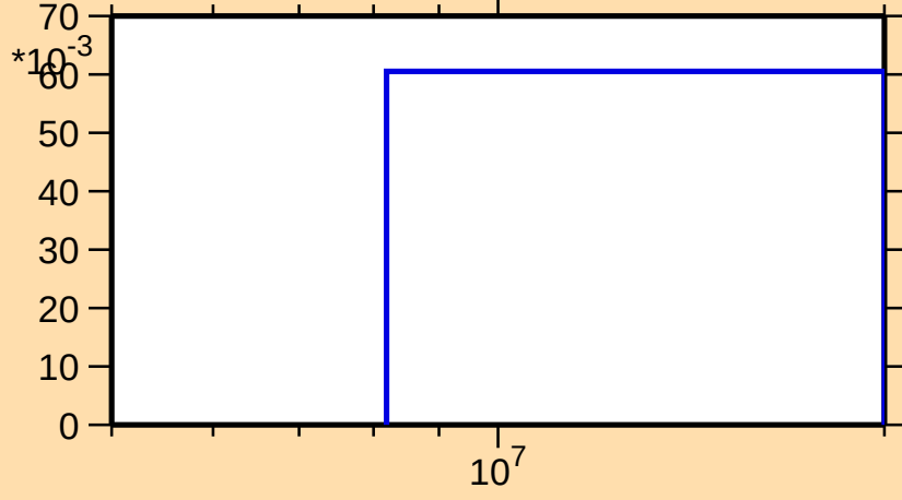
\sigma vs. E for ^{246}\text{Cf}(n,3n)
