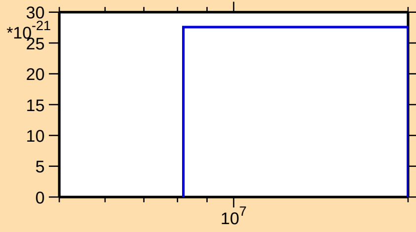
\sigma vs. E for ^{246}\text{Cf}(\text{mt } 42)
