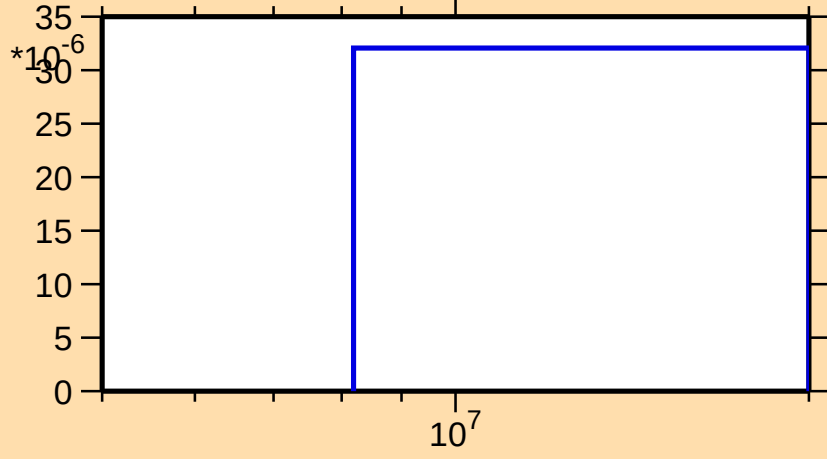
\sigma vs. E for ^{246}\text{Cf}(n,t)
