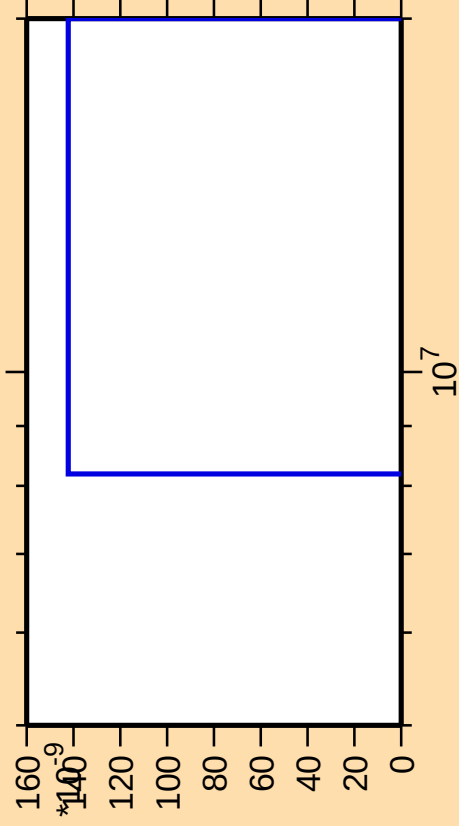
\Delta\sigma/\sigma vs. E for ^{246}\text{Cf}(\text{mt } 42)
