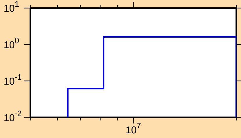
\sigma vs. E for ^{246}\text{Cf}(n,2n)
