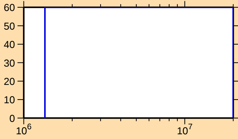
\Delta\sigma/\sigma vs. E for ^{250}\text{Cf}(n,n\text{cont.})
