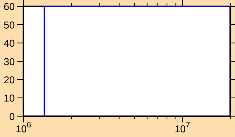
\Delta\sigma/\sigma vs. E for ^{250}\text{Cf}(n,n\text{cont.})
