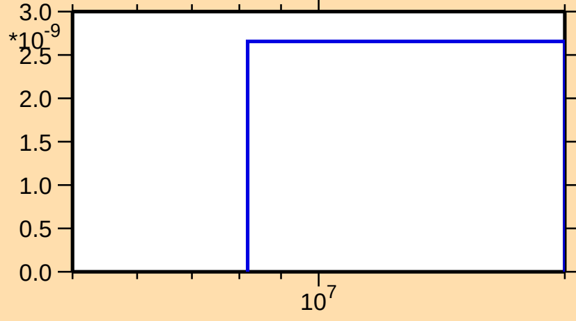
\sigma vs. E for ^{250}\text{Cf}(n,2n\alpha)
