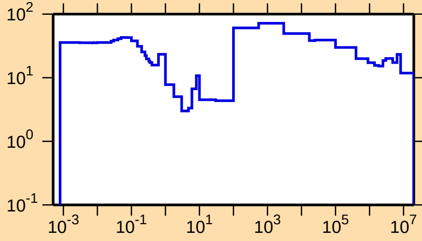
\Delta\sigma/\sigma vs. E for ^{250}\text{Cf}(n,el.)
