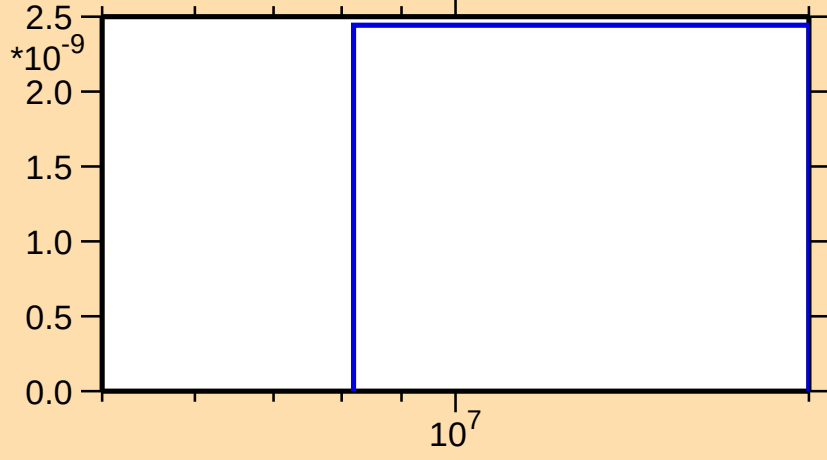
\sigma vs. E for ^{250}\text{Cf}(n,nd)
