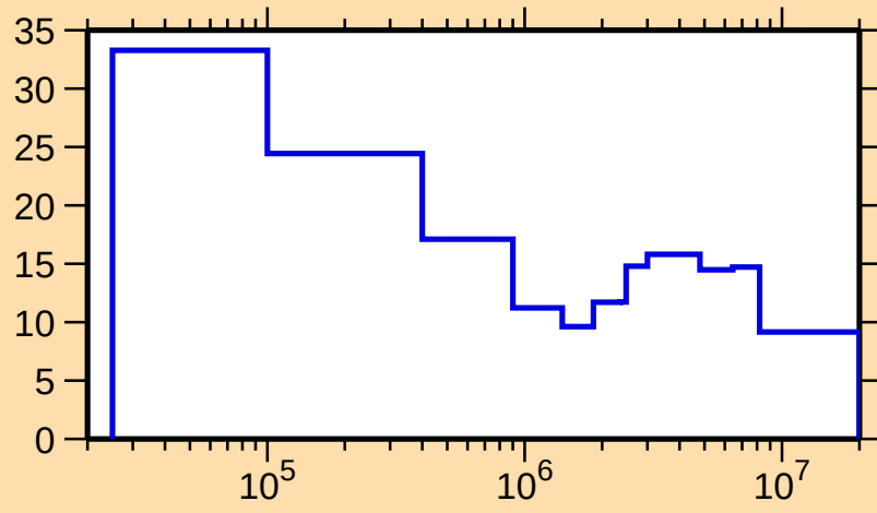
\Delta\sigma/\sigma vs. E for ^{250}\text{Cf}(n,\text{tot.})
