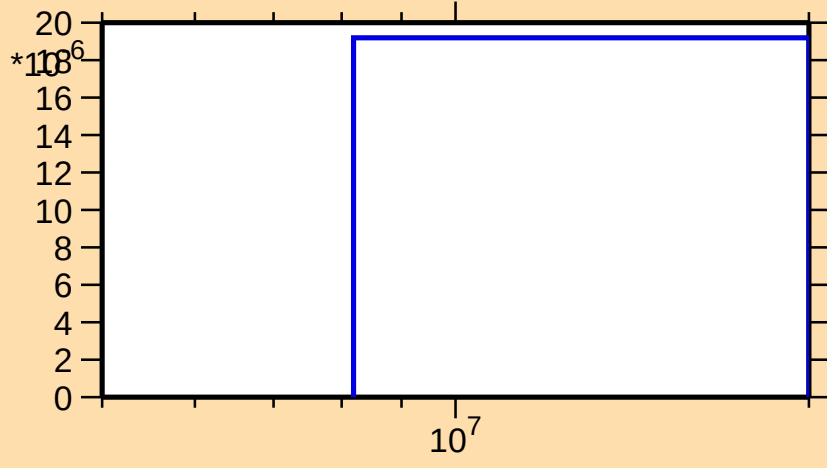
\sigma vs. E for ^{250}\text{Cf}(n,t)
