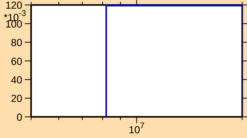
\sigma vs. E for ^{250}\text{Cf}(n,3n)
