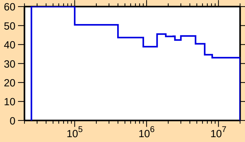
\Delta\sigma/\sigma vs. E for ^{250}\text{Cf}(n,n_1)
