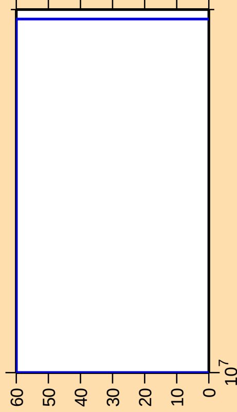
\Delta\sigma/\sigma vs. E for ^{254}\text{Cf}(n,\text{nd})
