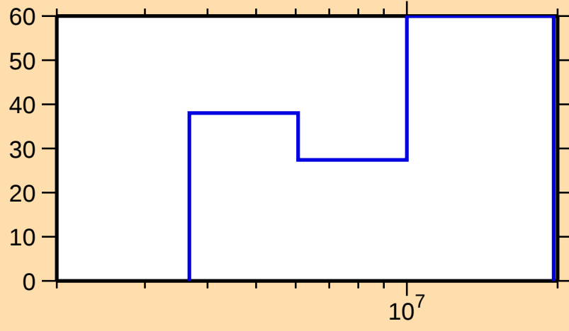
\Delta\sigma/\sigma vs. E for ^{254}\text{Cf}(n,\text{inel.})
