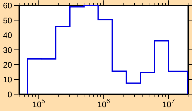
\Delta\sigma/\sigma vs. E for ^{254}\text{Cf}(n,\text{el.})
