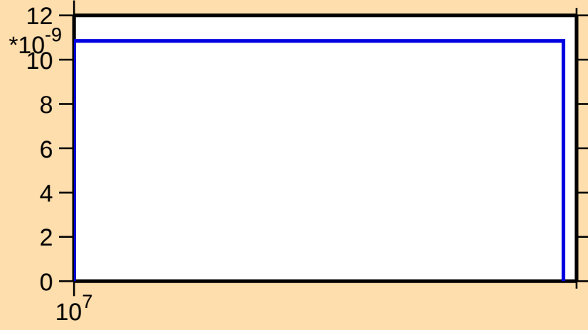
\sigma vs. E for ^{254}\text{Cf}(n,nt)
