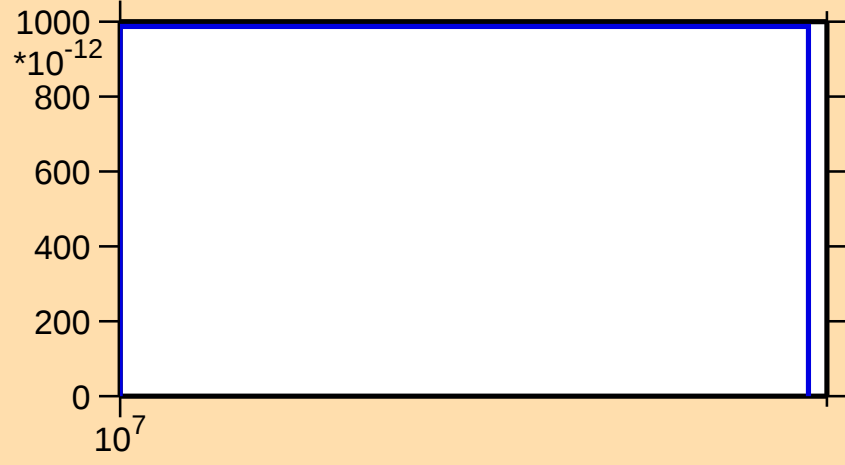
\sigma vs. E for ^{254}\text{Cf}(n,\text{nd})
