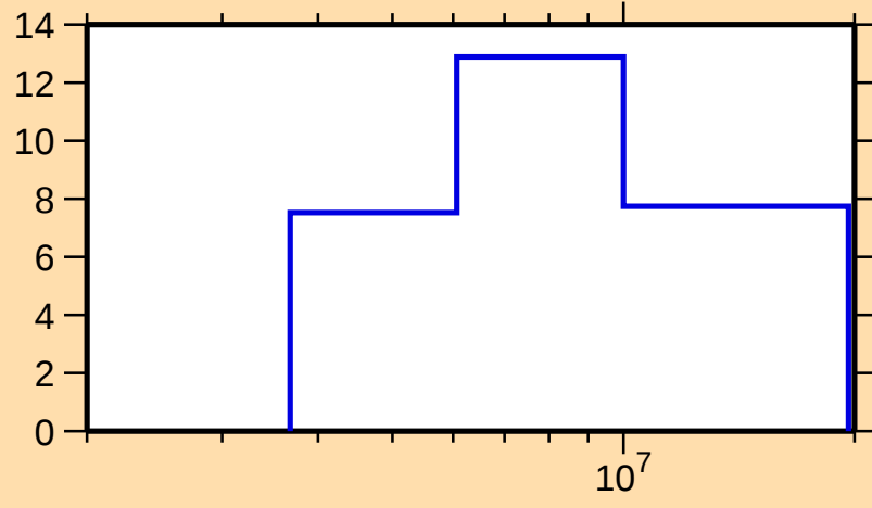
\Delta\sigma/\sigma vs. E for ^{254}\text{Cf}(n,\text{tot.})
