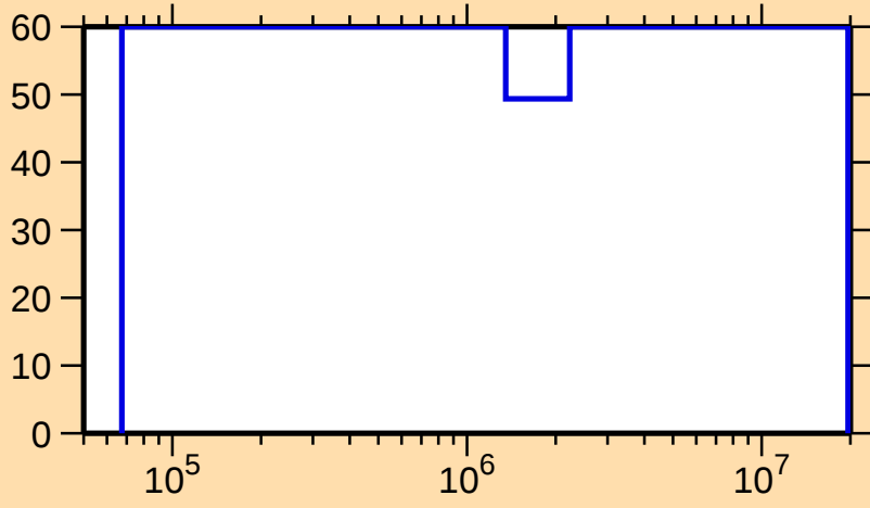
\Delta\sigma/\sigma vs. E for ^{254}\text{Cf}(n,n_1)
