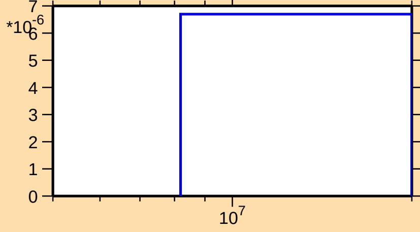
\sigma vs. E for ^{254}\text{Cf}(n,np)
