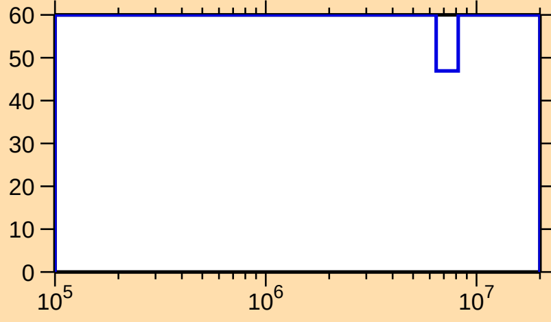
\Delta\sigma/\sigma vs. E for ^{254}\text{Cf}(n,ncont.)
