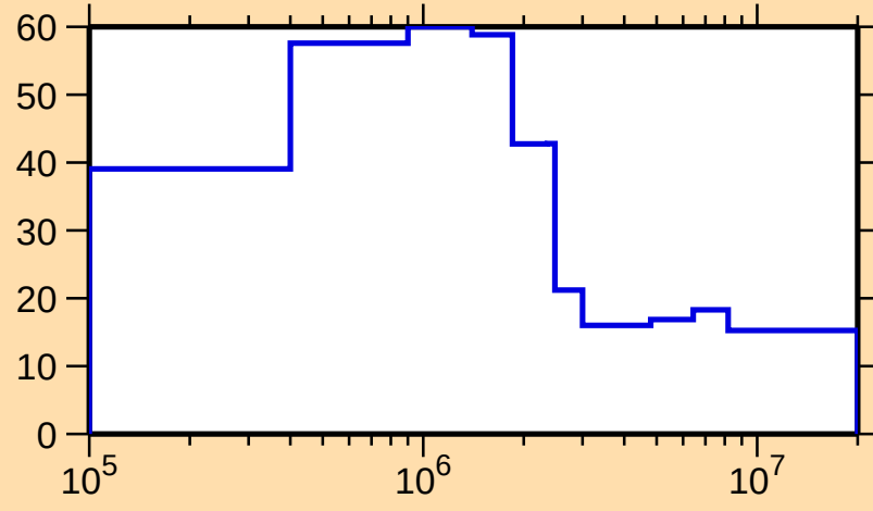
\Delta\sigma/\sigma vs. E for ^{254}\text{Cf}(n,\text{nonel.})
