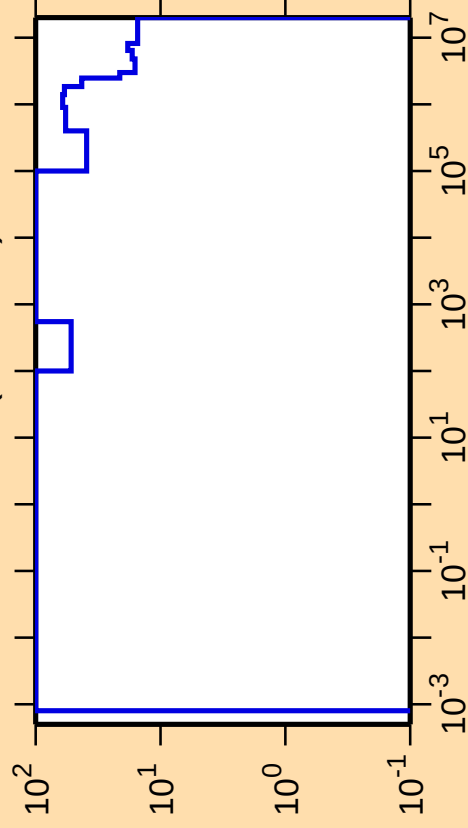
\Delta\sigma/\sigma vs. E for ^{254}\text{Cf}(n,\text{nonel.})
