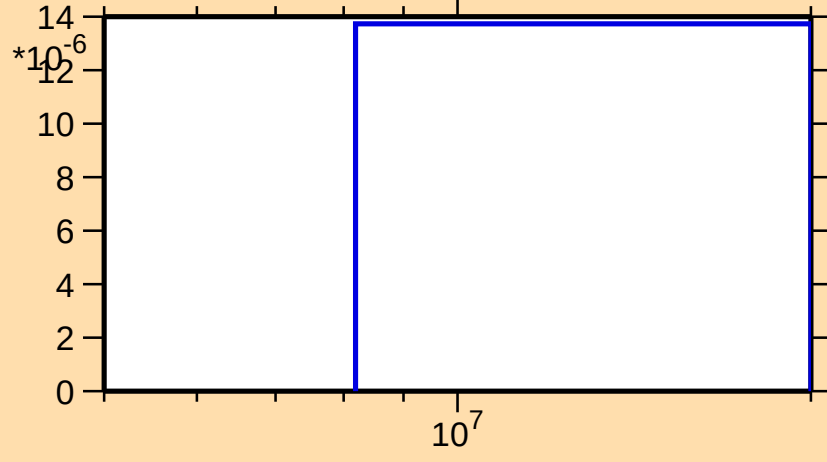
\sigma vs. E for ^{254}\text{Cf}(n,d)
