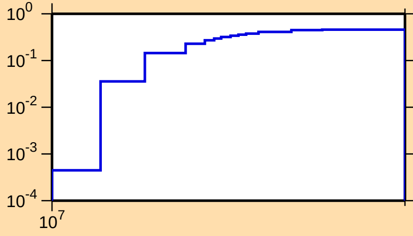
\sigma vs. E for ^{255}\text{Cf}(n,3n)
