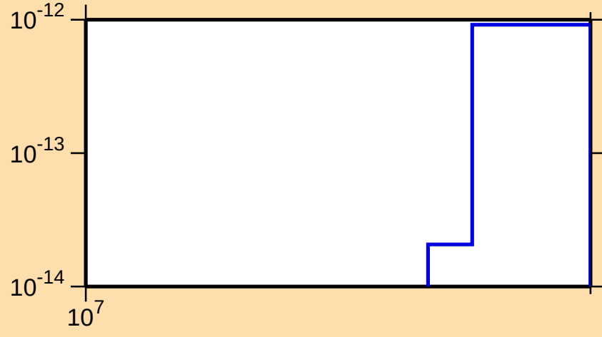
\sigma vs. E for ^{255}\text{Cf}(n,\text{He3})
