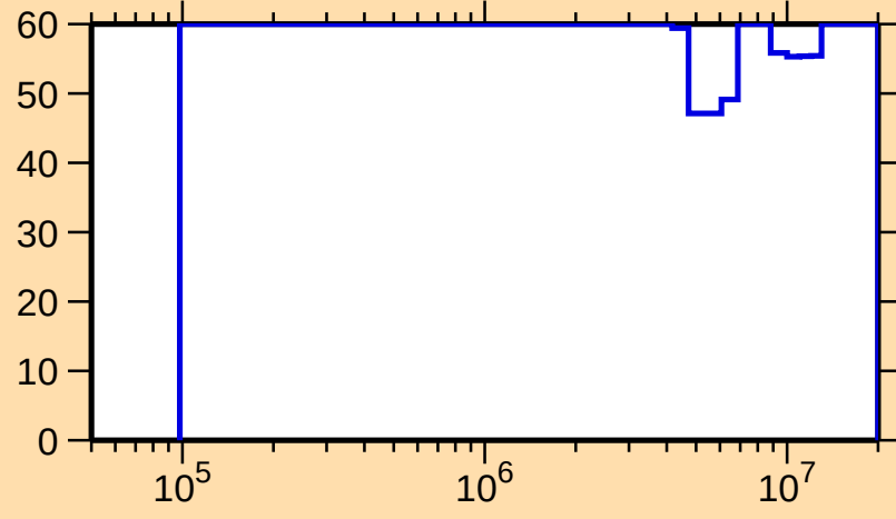
\Delta\sigma/\sigma vs. E for ^{255}\text{Cf}(n,n_1)
