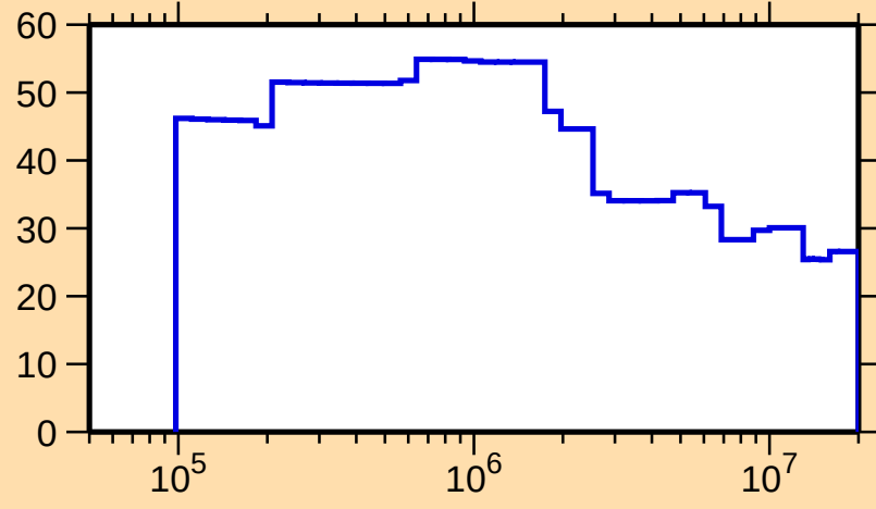
\Delta\sigma/\sigma vs. E for ^{255}\text{Cf}(n,\text{nonel.})
