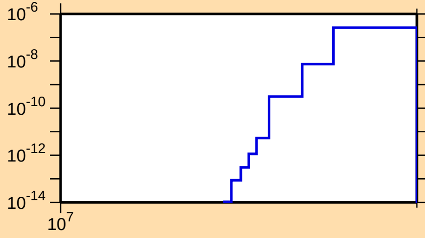
\sigma vs. E for ^{255}\text{Cf}(n,2np)
