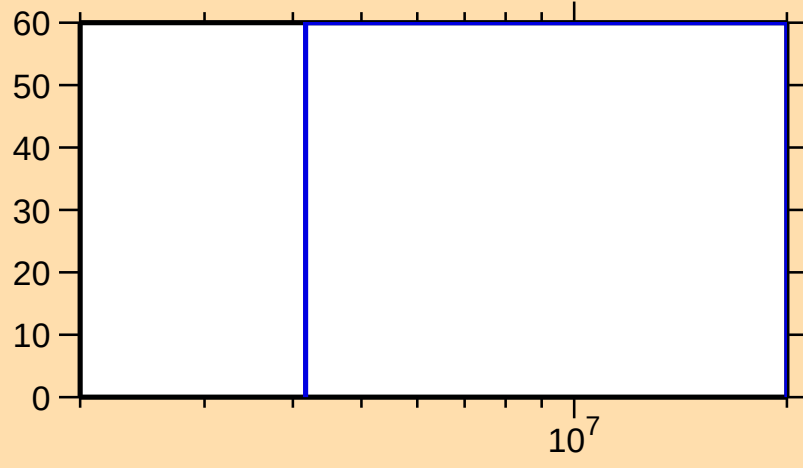
\Delta\sigma/\sigma vs. E for ^{255}\text{Cf}(n,\text{inel.})
