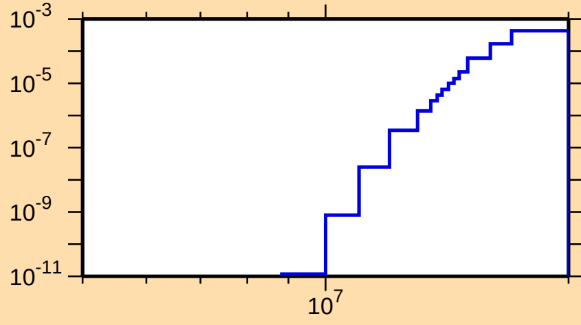
\sigma vs. E for ^{255}\text{Cf}(n,t)
