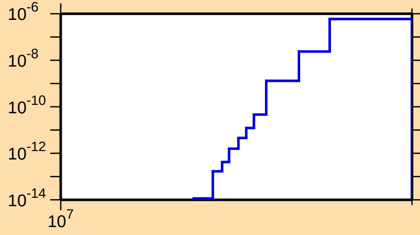
\sigma vs. E for ^{255}\text{Cf}(n,nd)
