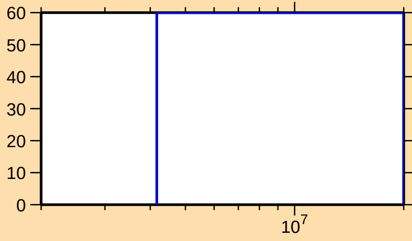
\Delta\sigma/\sigma vs. E for ^{255}\text{Cf}(n,2n)
