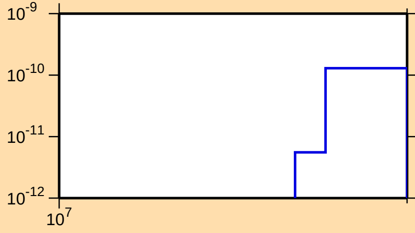
\sigma vs. E for ^{255}\text{Cf}(n,3n\alpha)
