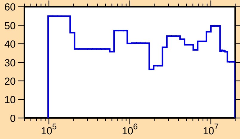
\Delta\sigma/\sigma vs. E for ^{255}\text{Cf}(n,\text{el.})
