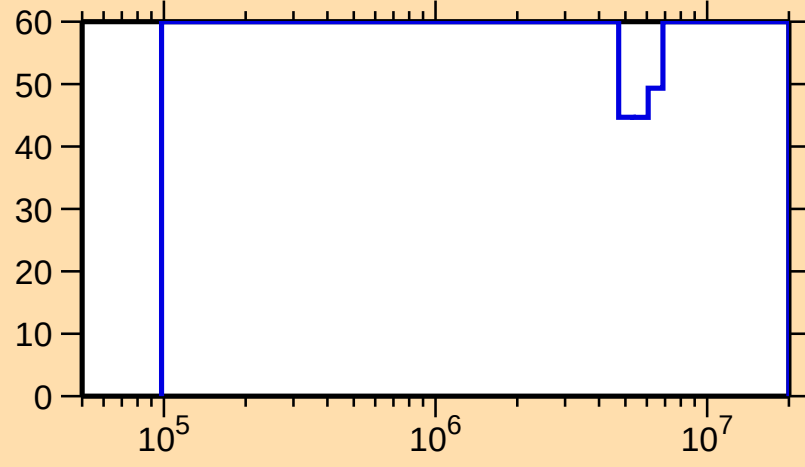
\Delta\sigma/\sigma vs. E for ^{255}\text{Cf}(n,f)
