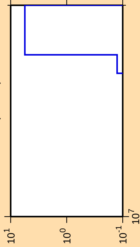
\Delta\sigma/\sigma vs. E for ^{255}\text{Cf}(n,\text{He3})
