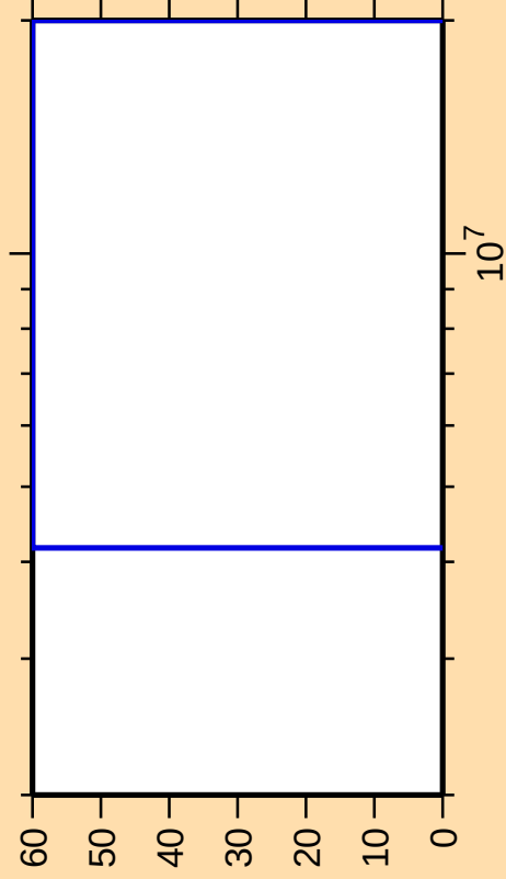
\Delta\sigma/\sigma vs. E for ^{255}\text{Cf}(n,\gamma)
