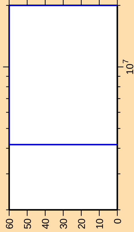
\Delta\sigma/\sigma vs. E for ^{255}\text{Cf}(n,2n)
