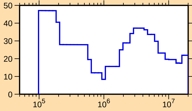
\Delta\sigma/\sigma vs. E for ^{255}\text{Cf}(n,\text{tot.})
