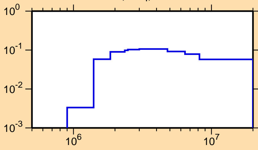
\sigma vs. E for ^{34}\text{Cl}(n,n_4)
