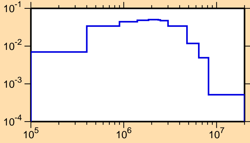
\sigma vs. E for ^{34}\text{Cl}(n,n_1)
