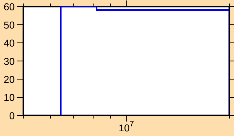
\Delta\sigma/\sigma vs. E for ^{42}\text{Cl}(n,\gamma)
