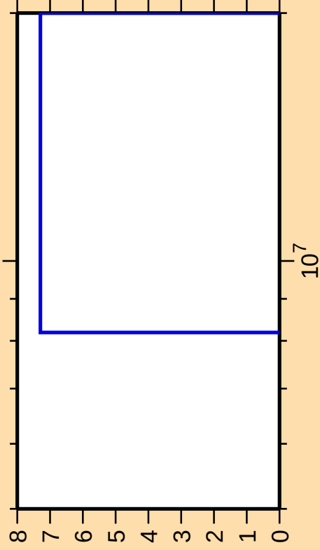
\Delta\sigma/\sigma vs. E for ^{42}\text{Cl}(n,2n\alpha)
