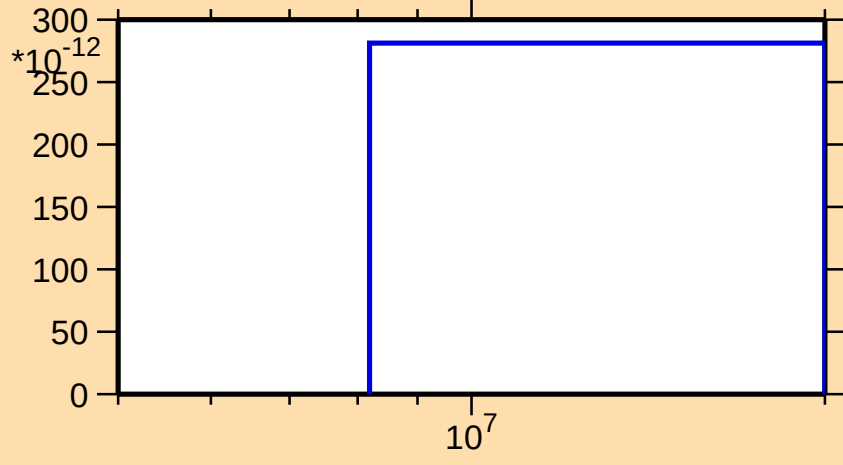
\sigma vs. E for ^{42}\text{Cl}(n,2np)
