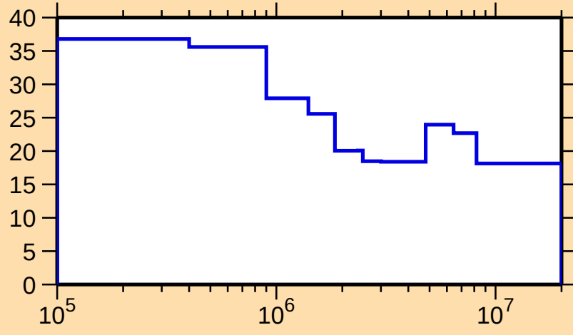
\Delta\sigma/\sigma vs. E for ^{42}\text{Cl}(n,\text{nonel.})
