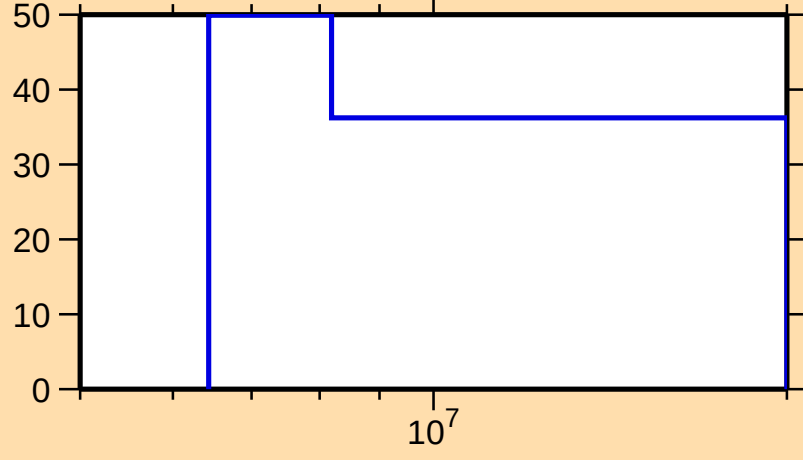
\Delta\sigma/\sigma vs. E for ^{42}\text{Cl}(n,2n)
