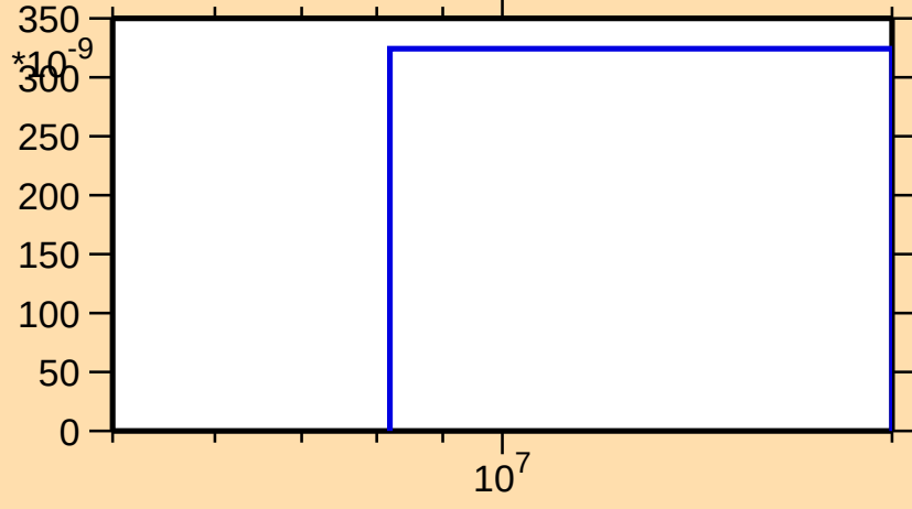
\sigma vs. E for ^{42}\text{Cl}(n,\text{nd})
