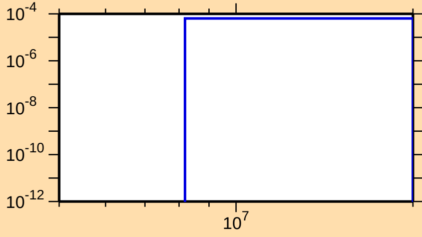
\sigma vs. E for ^{42}\text{Cl}(n,\alpha)
