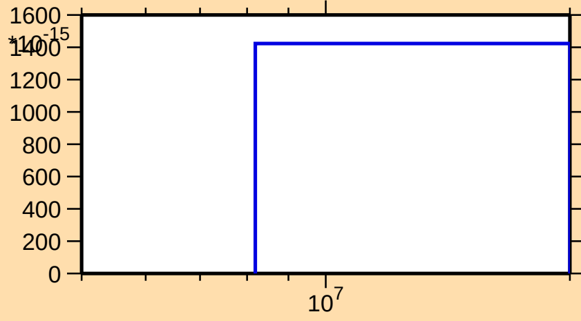
\sigma vs. E for ^{42}\text{Cl}(n,2n\alpha)
