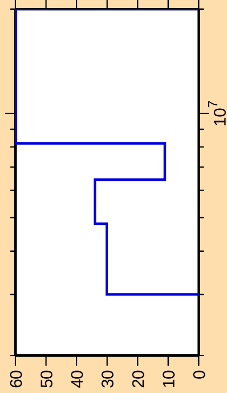
\Delta\sigma/\sigma vs. E for ^{42}\text{Cl}(n,\text{ncont.})
