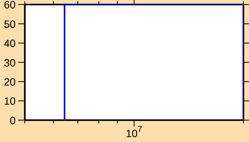
\Delta\sigma/\sigma vs. E for ^{42}\text{Cl}(n,n_1)
