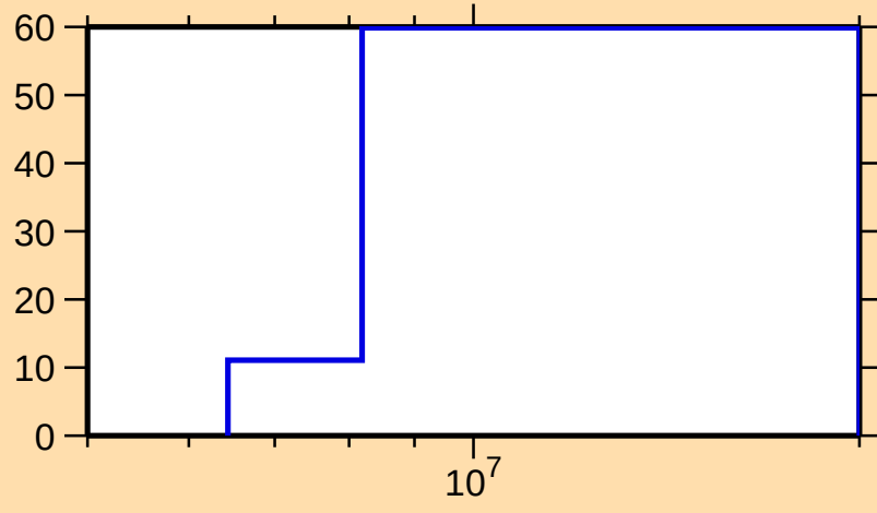
\Delta\sigma/\sigma vs. E for ^{42}\text{Cl}(n,n\text{cont.})
