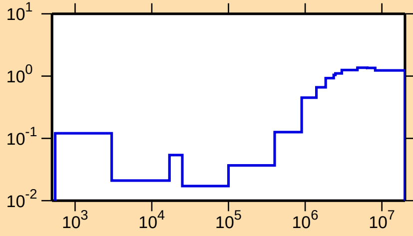
\sigma vs. E for ^{42}\text{Cl}(n,\text{nonel.})
