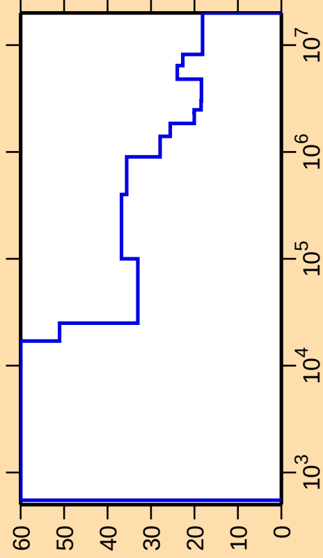
\Delta\sigma/\sigma vs. E for ^{42}\text{Cl}(n,\text{nonel.})
