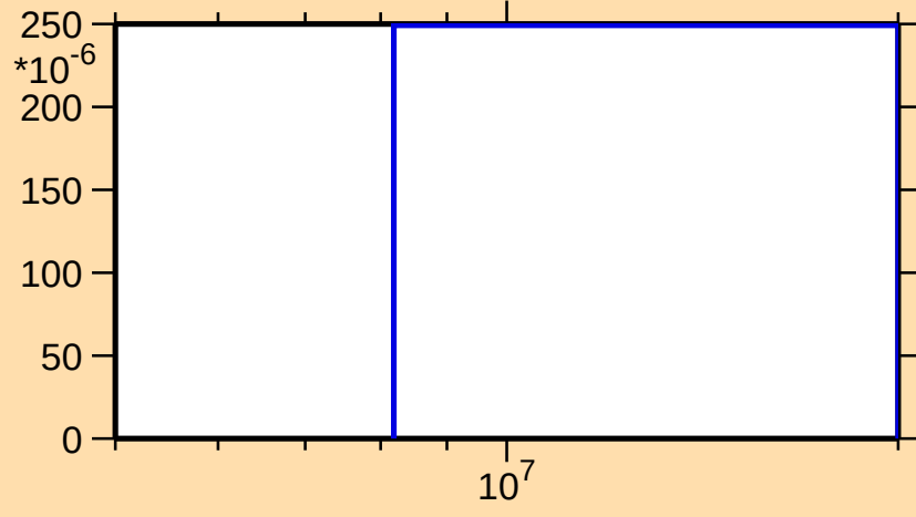
\sigma vs. E for ^{42}\text{Cl}(n,t)
