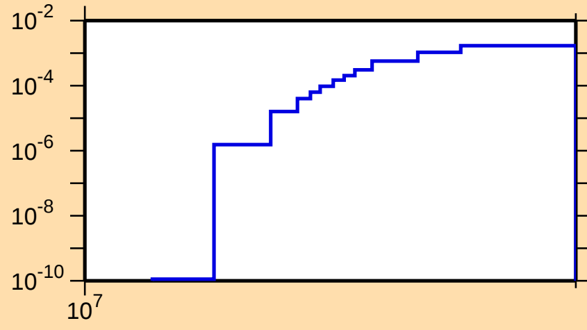
\sigma vs. E for ^{43}\text{Cl}(n,p)
