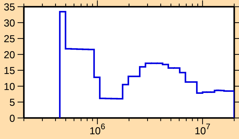
\Delta\sigma/\sigma vs. E for ^{43}\text{Cl}(n,\text{tot.})
