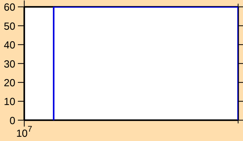
\Delta\sigma/\sigma vs. E for ^{43}\text{Cl}(n,\gamma)
