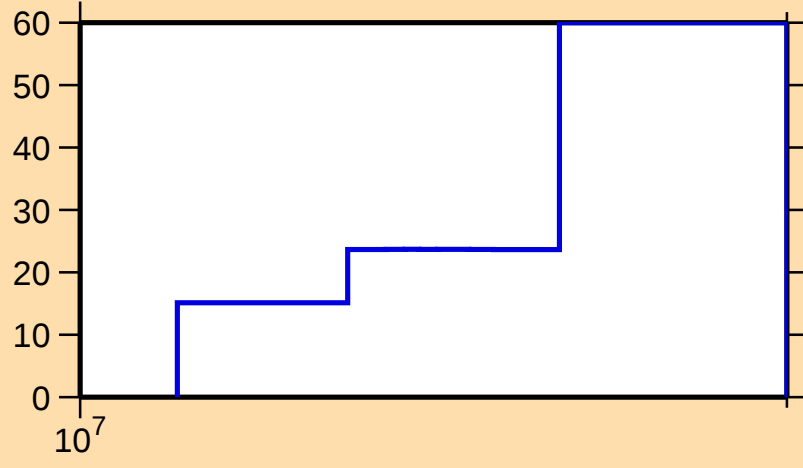
\Delta\sigma/\sigma vs. E for ^{43}\text{Cl}(n,2n)
