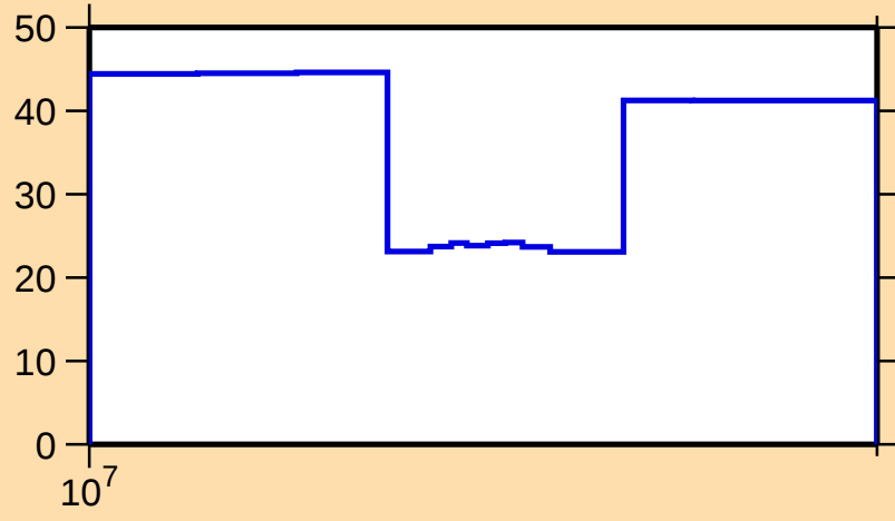
\Delta\sigma/\sigma vs. E for ^{43}\text{Cl}(n,n\text{cont.})
