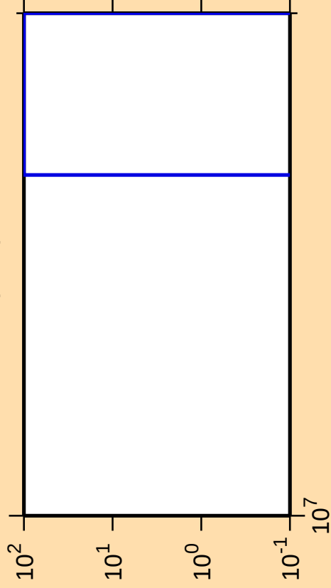
\Delta\sigma/\sigma vs. E for ^{43}\text{Cl}(n,\text{nt})
