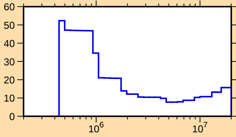
\Delta\sigma/\sigma vs. E for ^{43}\text{Cl}(n,\text{nonel.})
