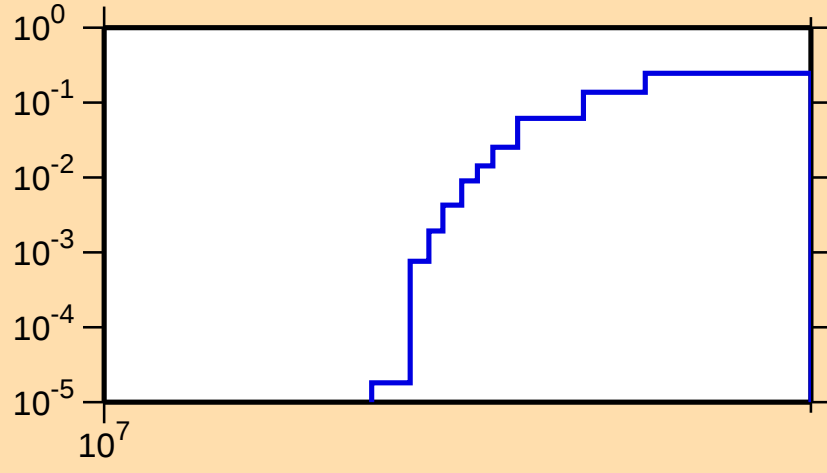
\sigma vs. E for ^{43}\text{Cl}(n,3n)
