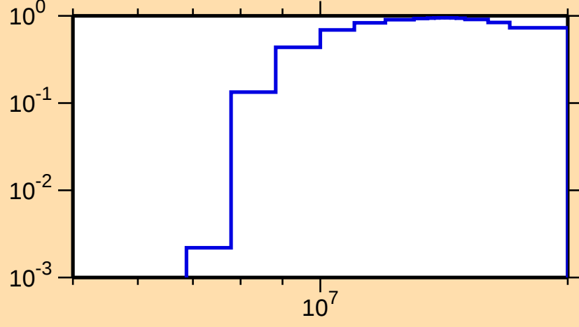
\sigma vs. E for ^{43}\text{Cl}(n,2n)
