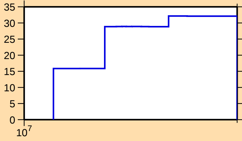
\Delta\sigma/\sigma vs. E for ^{43}\text{Cl}(n,\text{el.})
