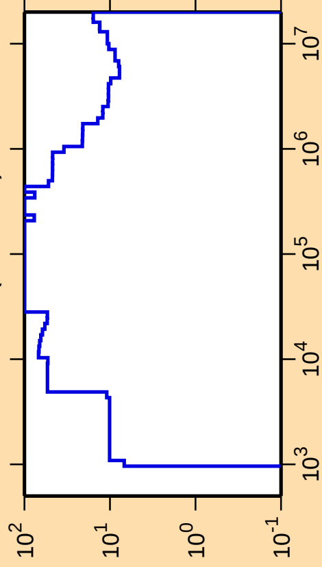
\Delta\sigma/\sigma vs. E for ^{43}\text{Cl}(n,\text{nonel.})
