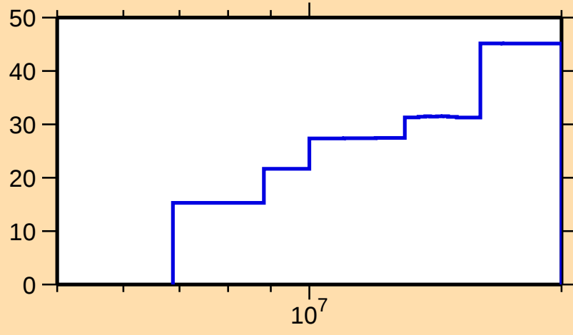
\Delta\sigma/\sigma vs. E for ^{43}\text{Cl}(n,\text{inel.})
