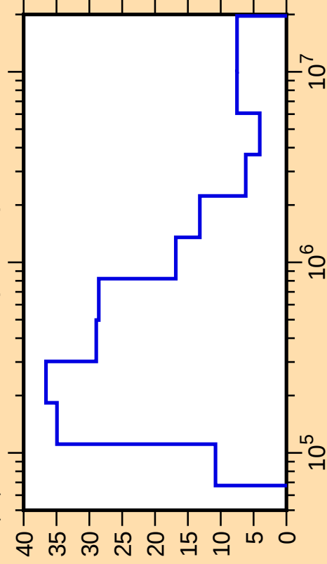
\Delta\mu/\mu vs. E for ^{43}\text{Cl}(\text{mt251})
