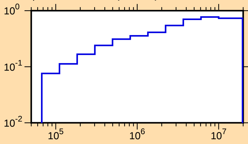
\mu vs. E for ^{43}\text{Cl}(\text{mt251})
