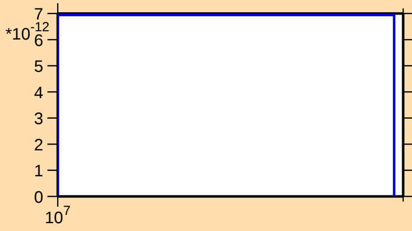
\sigma vs. E for ^{43}\text{Cl}(n,\text{nd})
