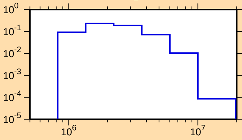
\sigma vs. E for ^{43}\text{Cl}(n,n_2)
