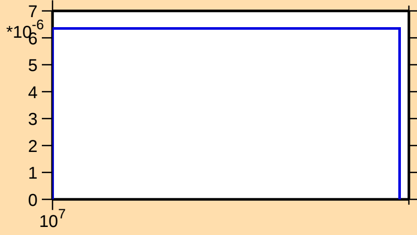
\sigma vs. E for ^{43}\text{Cl}(n,t)
