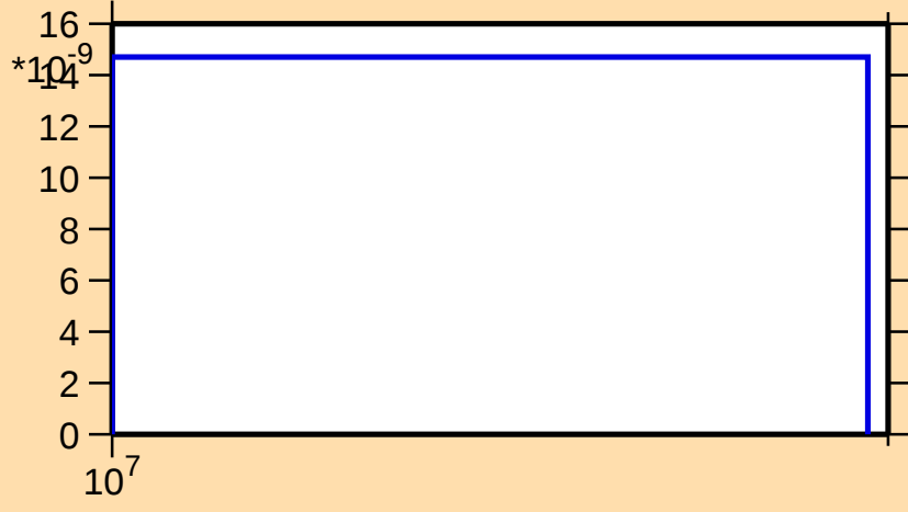
\sigma vs. E for ^{43}\text{Cl}(n,n\alpha)
