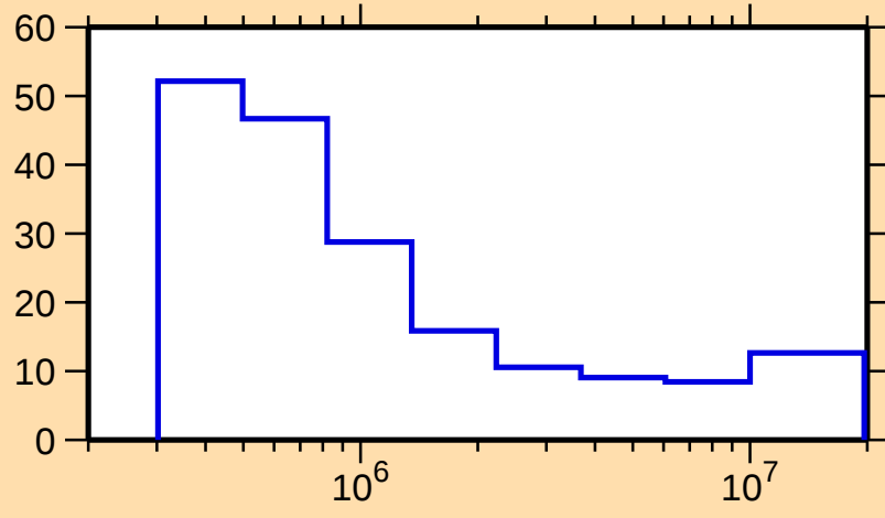
\Delta\sigma/\sigma vs. E for ^{43}\text{Cl}(\text{n,nonel.})
