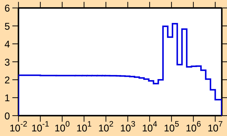
\sigma vs. E for ^{43}\text{Cl}(n,\text{el.})
