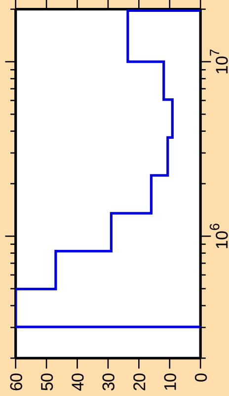
\Delta\sigma/\sigma vs. E for ^{43}\text{Cl}(\text{n,inel.})
