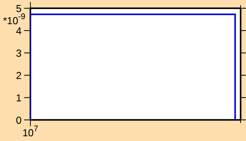
\sigma vs. E for ^{43}\text{Cl}(n,\text{nt})
