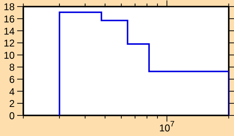
\Delta\sigma/\sigma vs. E for ^{43}\text{Cl}(\text{n},\text{tot.})
