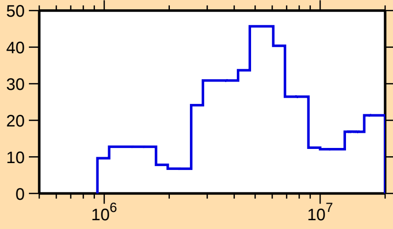
\Delta\sigma/\sigma vs. E for ^{241}\text{Cm}(n,\text{el.})
