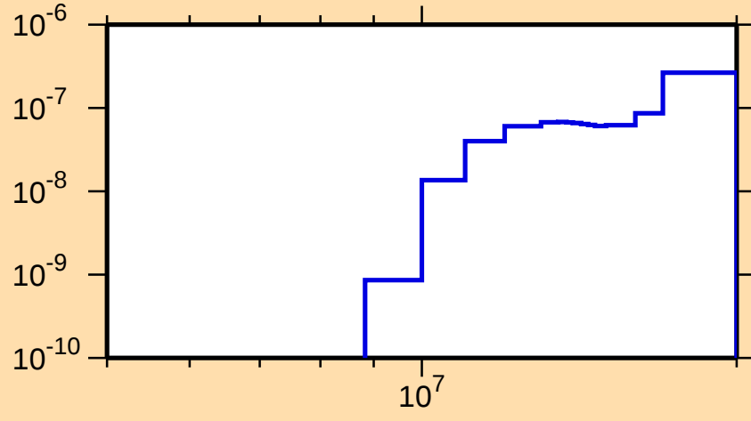
\sigma vs. E for ^{241}\text{Cm}(n,2n\alpha)
