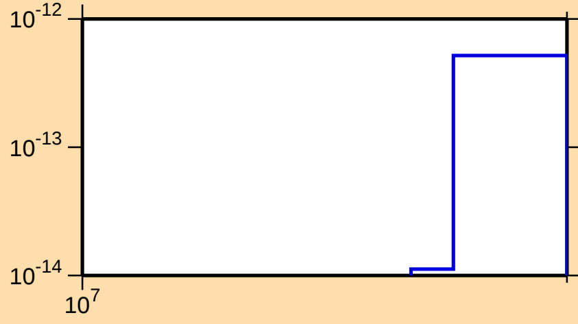
\sigma vs. E for ^{241}\text{Cm}(n,3n\alpha)
