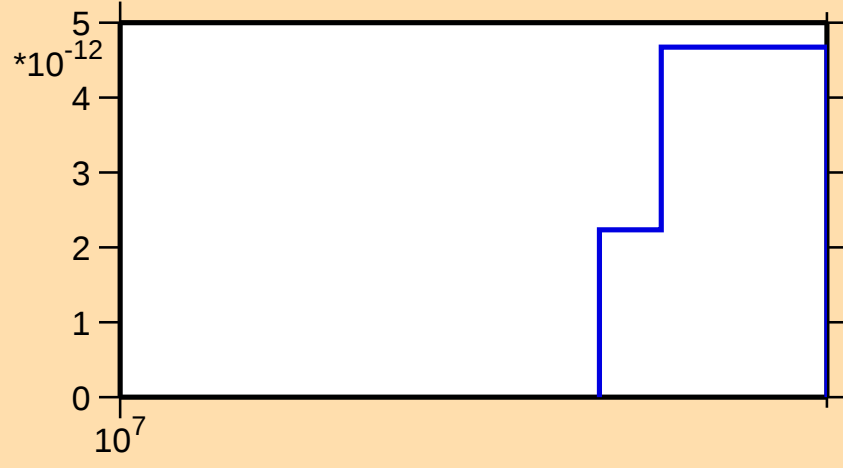
\sigma vs. E for ^{241}\text{Cm}(n,p\alpha)
