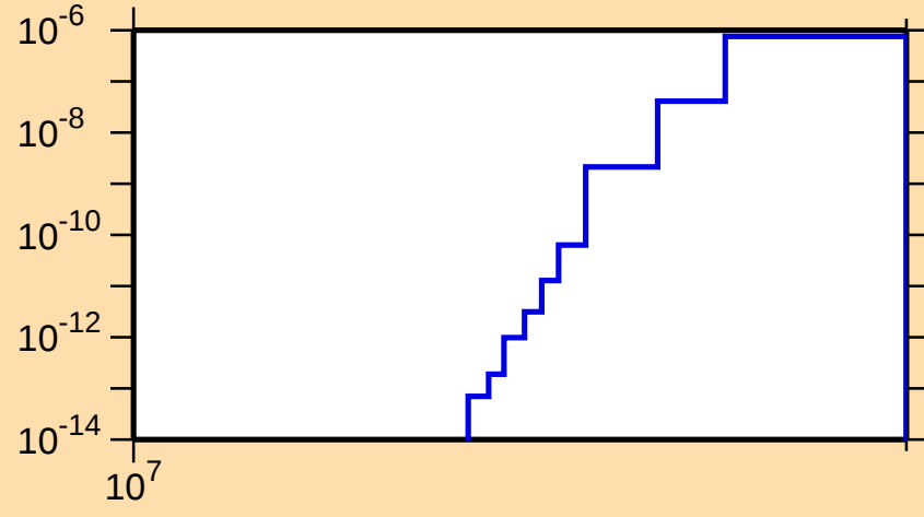
\sigma vs. E for ^{241}\text{Cm}(n,2np)
