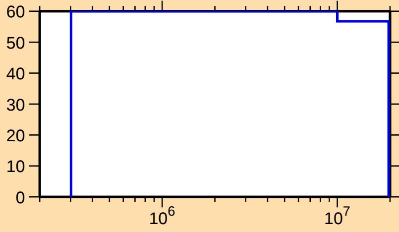
\Delta\sigma/\sigma vs. E for ^{241}\text{Cm}(n,n\text{cont.})
