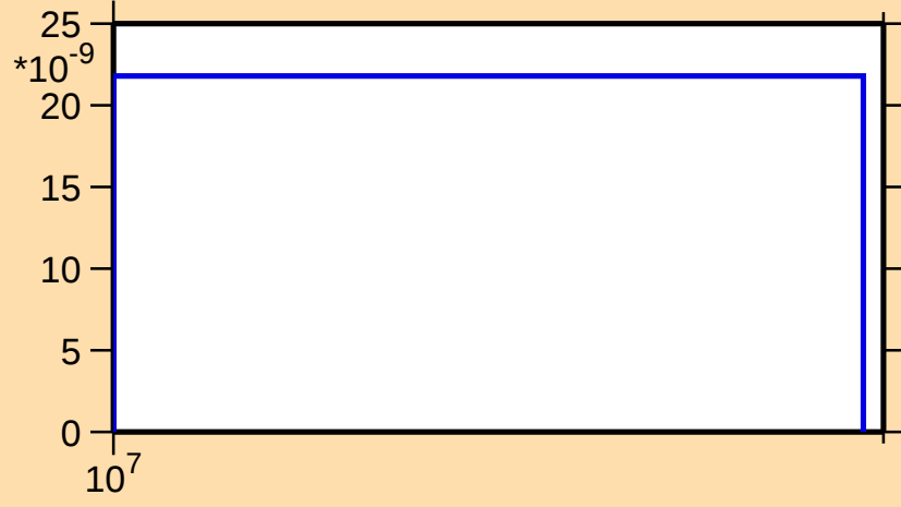
\sigma vs. E for ^{241}\text{Cm}(n,\text{nd})
