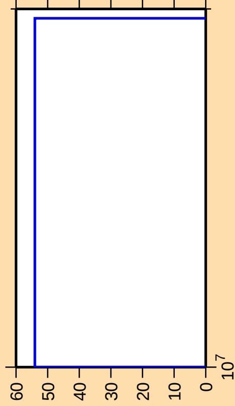
\Delta\sigma/\sigma vs. E for ^{241}\text{Cm}(n,\text{nd})
