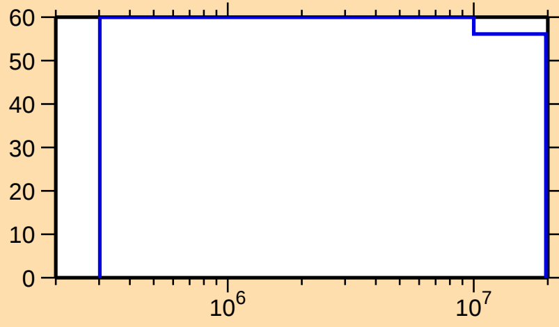
\Delta\sigma/\sigma vs. E for ^{241}\text{Cm}(\text{n},\text{inel.})
