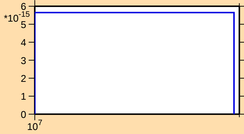
\sigma vs. E for ^{241}\text{Cm}(n,3n\alpha)
