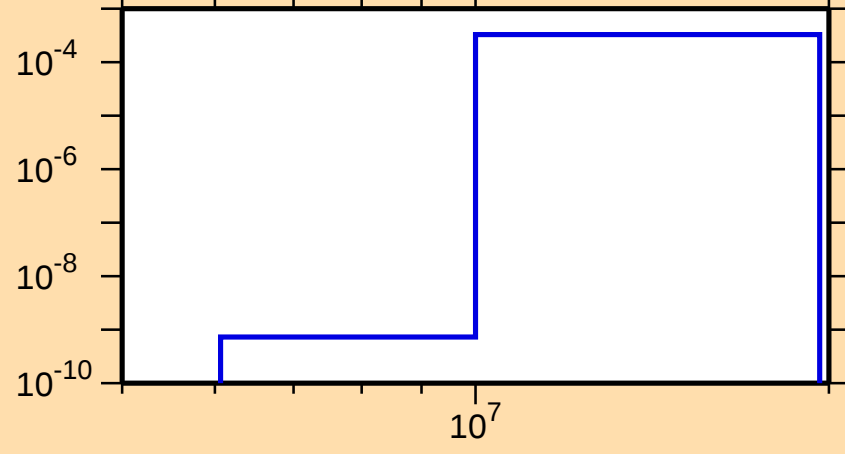
\sigma vs. E for ^{241}\text{Cm}(n,d)
