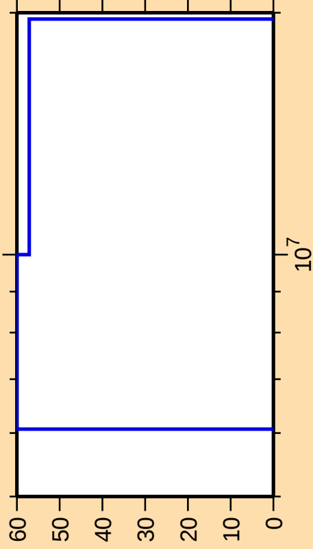
\Delta\sigma/\sigma vs. E for ^{241}\text{Cm}(n,p)
