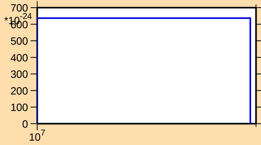
\sigma vs. E for ^{241}\text{Cm}(\text{mt } 42)
