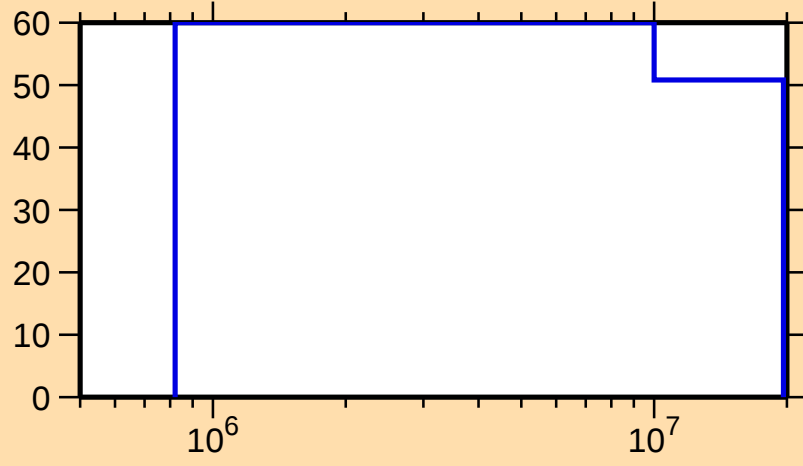
\Delta\sigma/\sigma vs. E for ^{241}\text{Cm}(n,\gamma)
