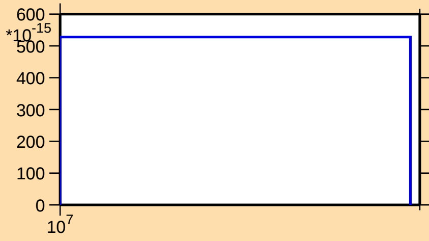
\sigma vs. E for ^{241}\text{Cm}(n,p\alpha)
