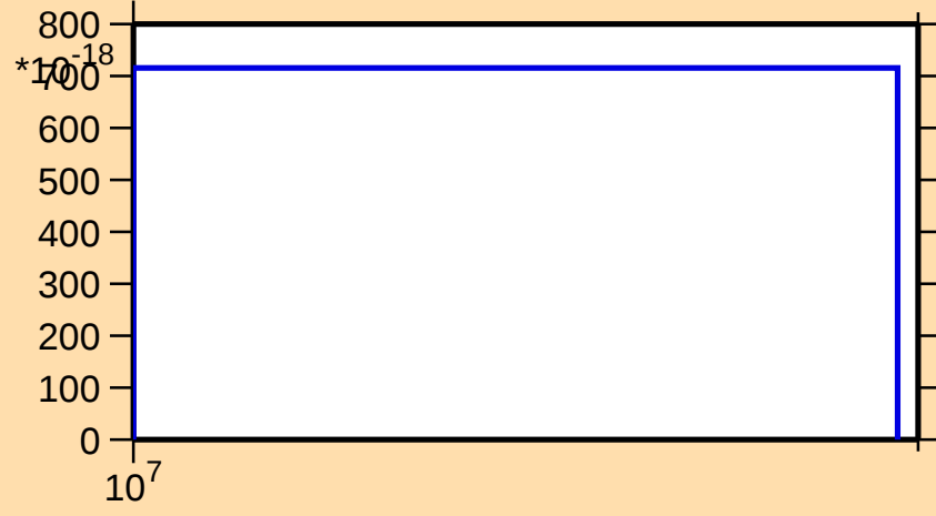
\sigma vs. E for ^{241}\text{Cm}(\text{mt } 34)
