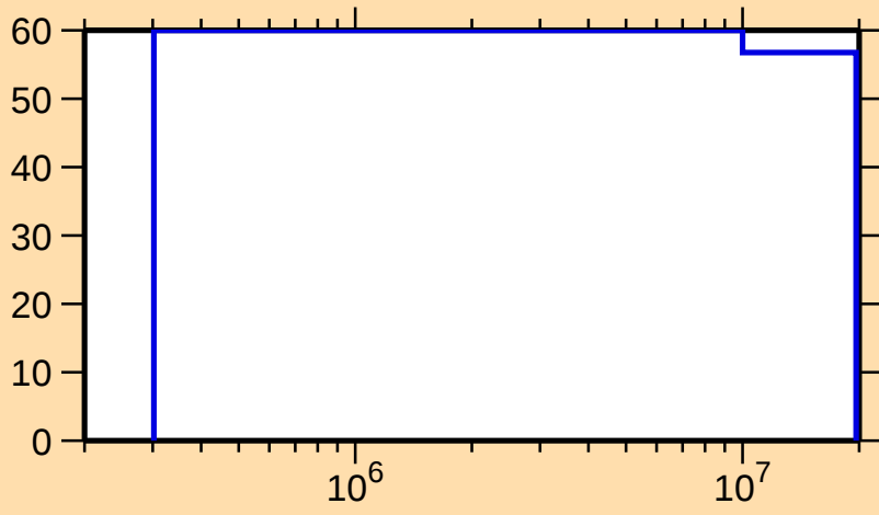
\Delta\sigma/\sigma vs. E for ^{241}\text{Cm}(n,n\text{cont.})
