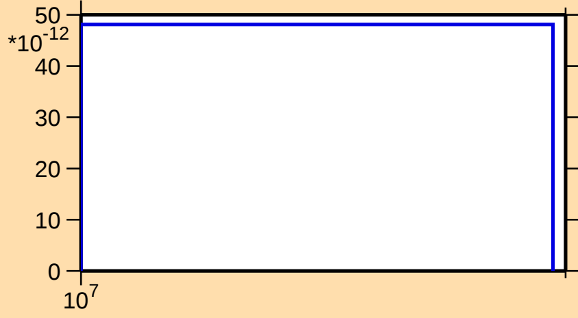
\sigma vs. E for ^{241}\text{Cm}(n,nt)
