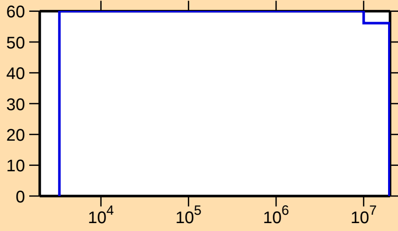
\Delta\sigma/\sigma vs. E for ^{241}\text{Cm}(n,\text{inel.})
