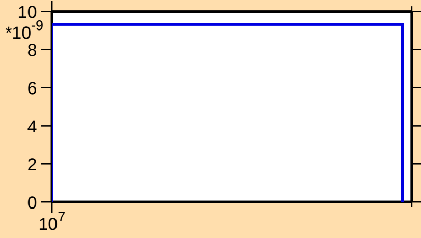
\sigma vs. E for ^{241}\text{Cm}(n,2np)
