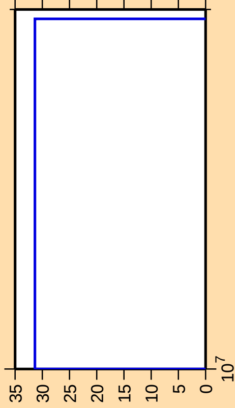
\Delta\sigma/\sigma vs. E for ^{241}\text{Cm}(n,\text{He}3)
