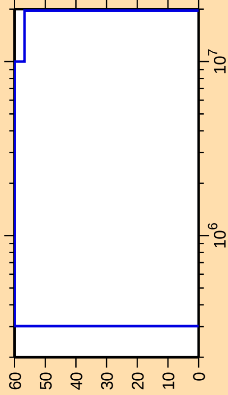
\Delta\sigma/\sigma vs. E for ^{241}\text{Cm}(n,n_{\text{cont}})
