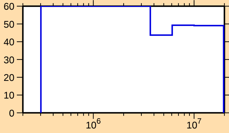
\Delta\sigma/\sigma vs. E for ^{241}\text{Cm}(n,n_1)
