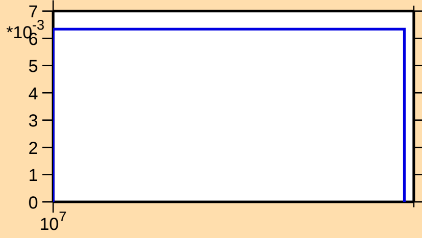
\sigma vs. E for ^{241}\text{Cm}(n,3n)
