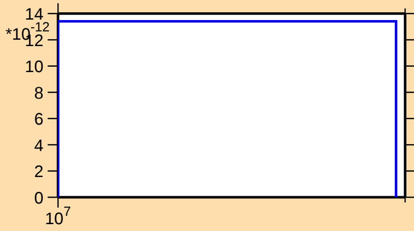
\sigma vs. E for ^{241}\text{Cm}(n,\text{He}3)
