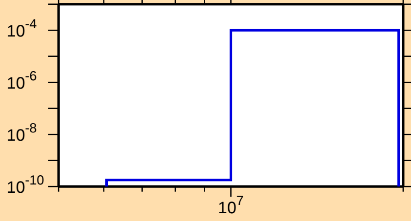
\sigma vs. E for ^{241}\text{Cm}(n,np)
