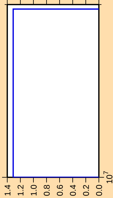
\Delta\sigma/\sigma vs. E for ^{241}\text{Cm}(n,p\alpha)
