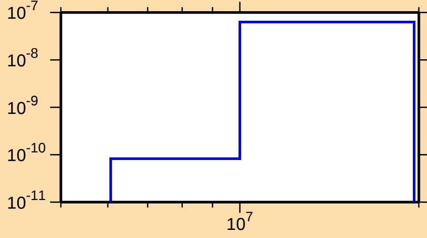
\sigma vs. E for ^{241}\text{Cm}(n,2n\alpha)
