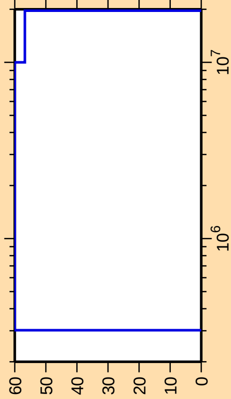
\Delta\sigma/\sigma vs. E for ^{241}\text{Cm}(\text{n},\text{ncont.})
