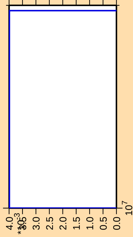
\Delta\sigma/\sigma vs. E for ^{241}\text{Cm}(\text{mt } 34)
