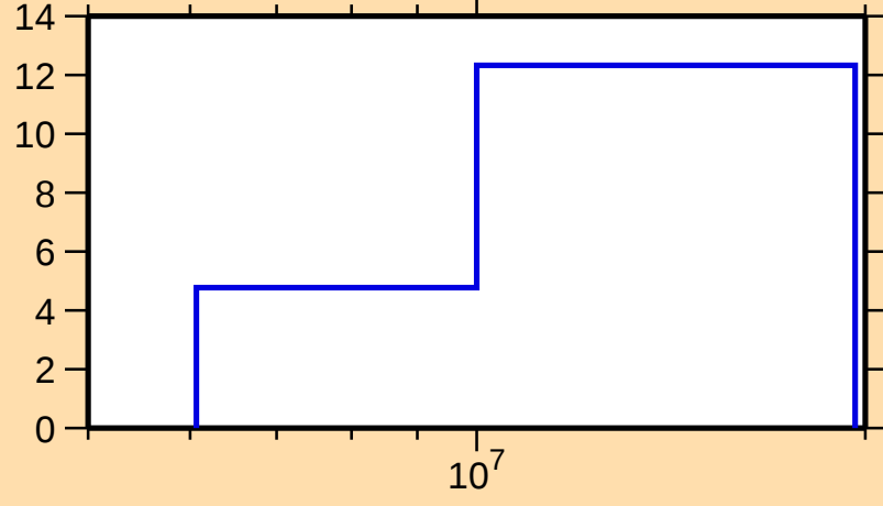
\Delta\sigma/\sigma vs. E for ^{241}\text{Cm}(n,\text{nonel.})
