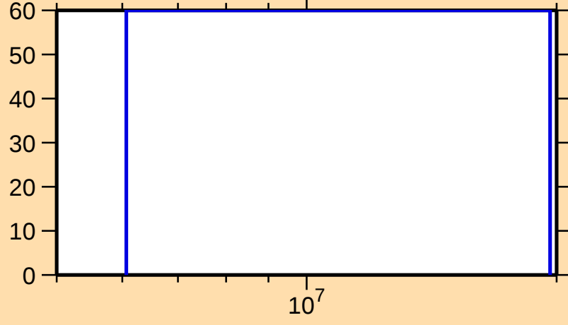
\Delta\sigma/\sigma vs. E for ^{241}\text{Cm}(n,2n)
