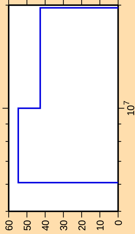
\Delta\sigma/\sigma vs. E for ^{241}\text{Cm}(n,d)
