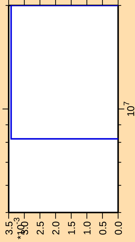
\Delta\sigma/\sigma vs. E for ^{241}\text{Cm}(n,3n\alpha)
