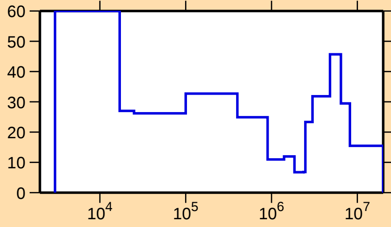
\Delta\sigma/\sigma vs. E for ^{241}\text{Cm}(\text{n,el.})
