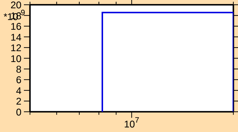
\sigma vs. E for ^{241}\text{Cm}(n,\text{nd})
