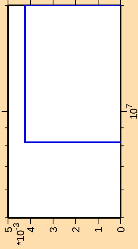
\Delta\sigma/\sigma vs. E for ^{241}\text{Cm}(\text{mt } 34)
