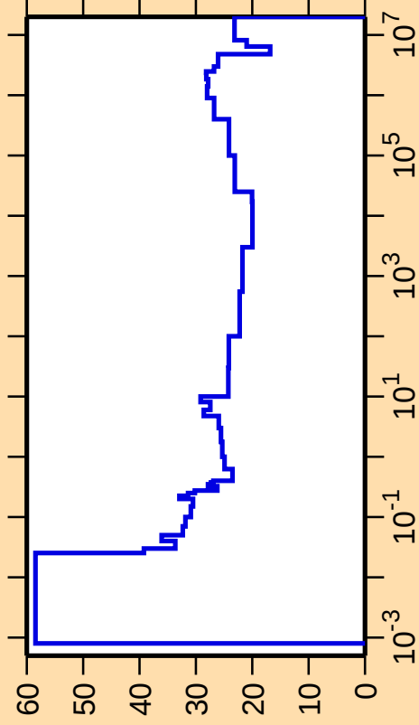
\Delta\sigma/\sigma vs. E for ^{243}\text{Cm}(n,\alpha)
