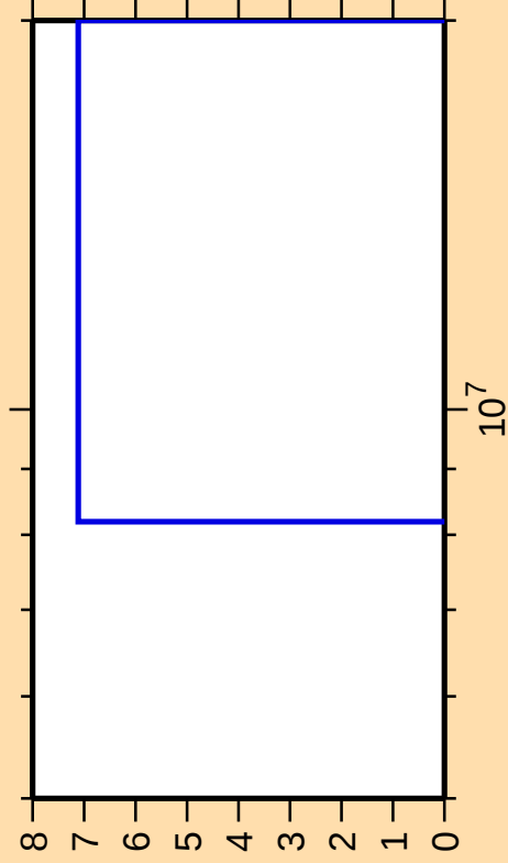
\Delta\sigma/\sigma vs. E for ^{243}\text{Cm}(n,3n\alpha)
