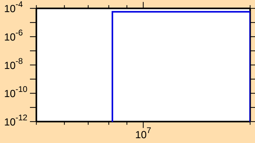
\sigma vs. E for ^{243}\text{Cm}(n,2n\alpha)
