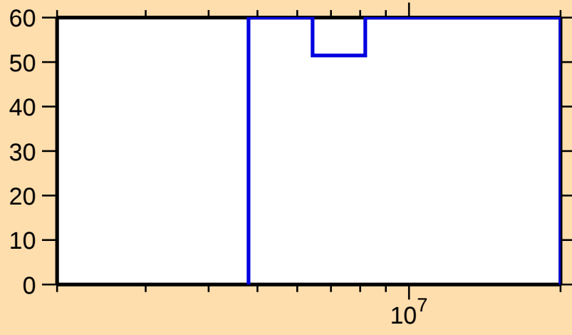
\Delta\sigma/\sigma vs. E for ^{243}\text{Cm}(n,2n)
