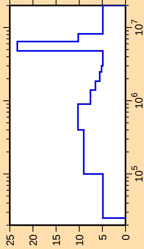
\Delta\sigma/\sigma vs. E for ^{243}\text{Cm}(\text{n,inel.})
