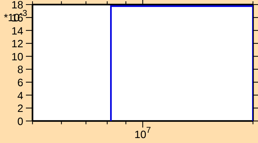
\sigma vs. E for ^{243}\text{Cm}(n,3n)
