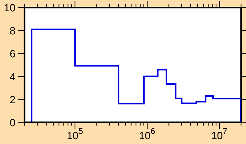
\Delta\sigma/\sigma vs. E for ^{243}\text{Cm}(\text{n,nonel.})
