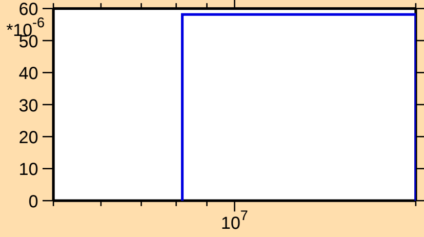
\sigma vs. E for ^{244}\text{Cm}(n,d)
