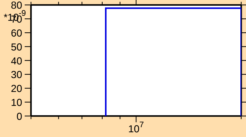
\sigma vs. E for ^{244}\text{Cm}(n,3n\alpha)
