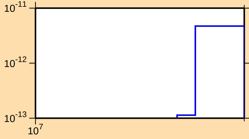
\sigma vs. E for ^{249}\text{Cm}(n,3n\alpha)
