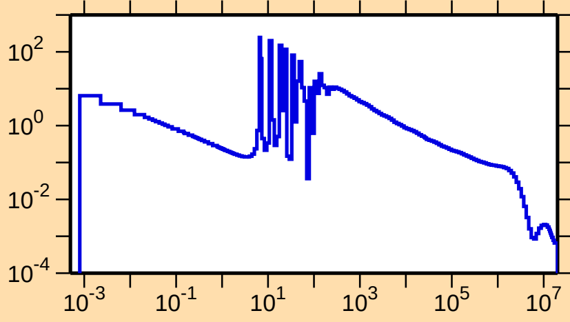
\sigma vs. E for ^{249}\text{Cm}(n,\gamma)
