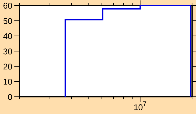
\Delta\sigma/\sigma vs. E for ^{249}\text{Cm}(n,2n)
