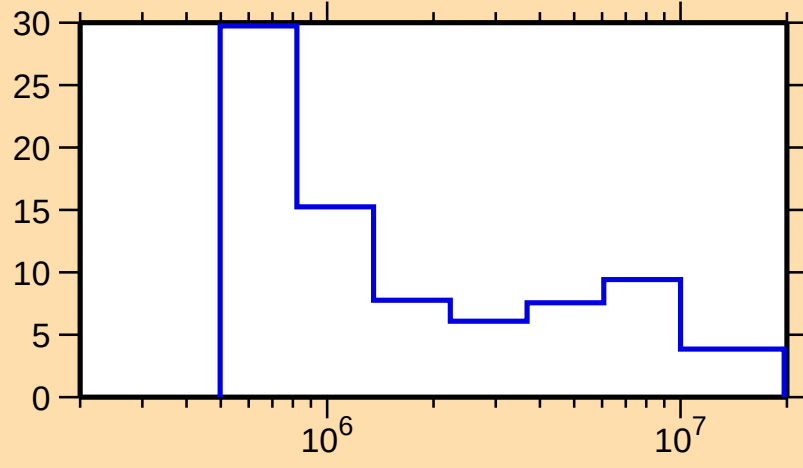
\Delta\sigma/\sigma vs. E for ^{249}\text{Cm}(n,\text{tot.})
