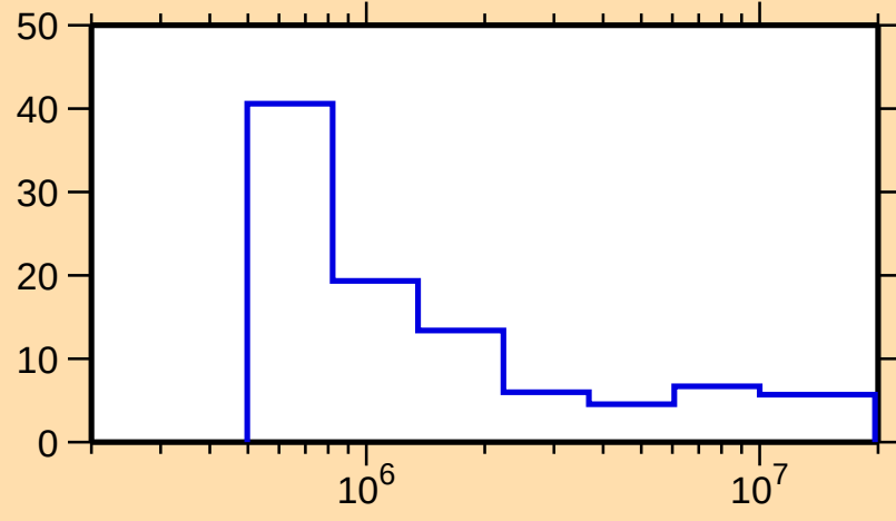
\Delta\sigma/\sigma vs. E for ^{249}\text{Cm}(n,\text{nonel.})
