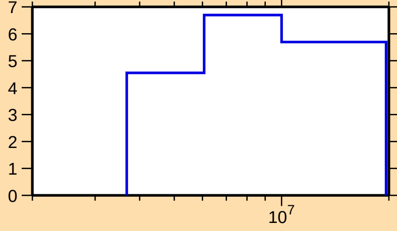
\Delta\sigma/\sigma vs. E for ^{249}\text{Cm}(n,\text{nonel.})
