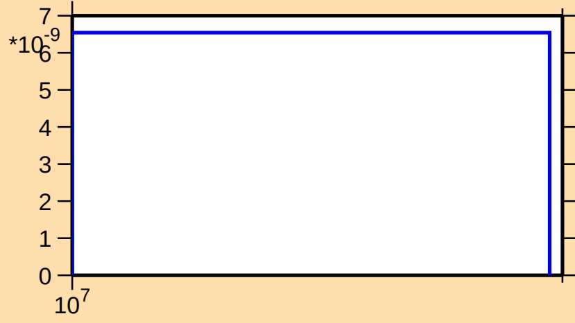
\sigma vs. E for ^{249}\text{Cm}(n,\text{nd})
