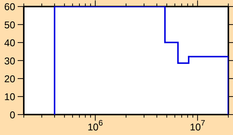
\Delta\sigma/\sigma vs. E for ^{249}\text{Cm}(n,f)
