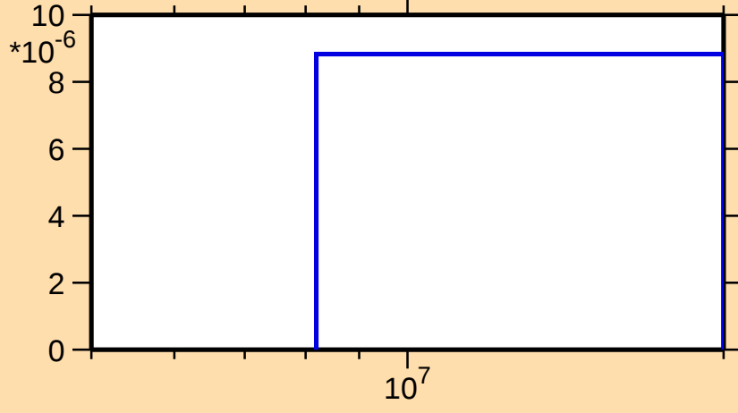
\sigma vs. E for ^{249}\text{Cm}(n,np)
