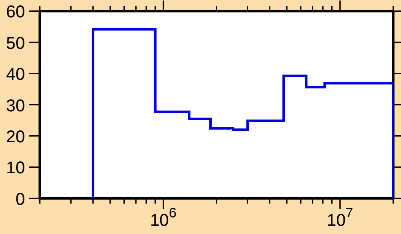
\Delta\sigma/\sigma vs. E for ^{249}\text{Cm}(n,\text{inel.})
