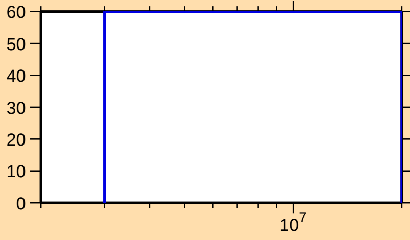
\Delta\sigma/\sigma vs. E for ^{249}\text{Cm}(n,\gamma)
