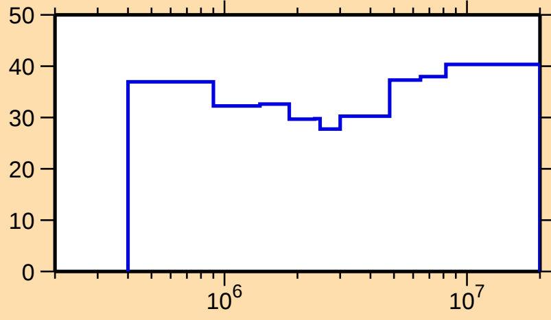
\Delta\sigma/\sigma vs. E for ^{249}\text{Cm}(n,n_1)
