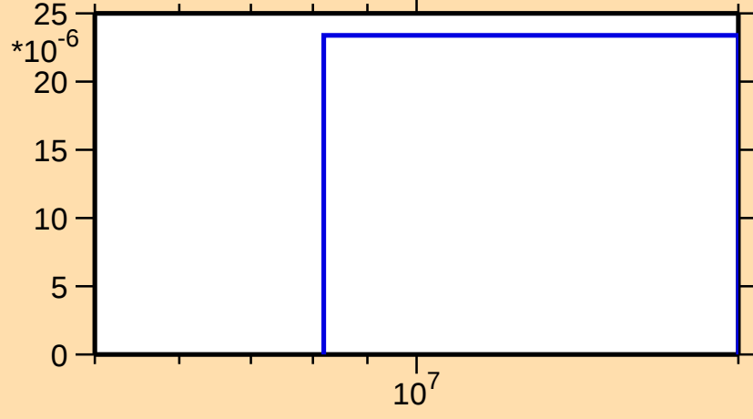
\sigma vs. E for ^{249}\text{Cm}(n,d)
