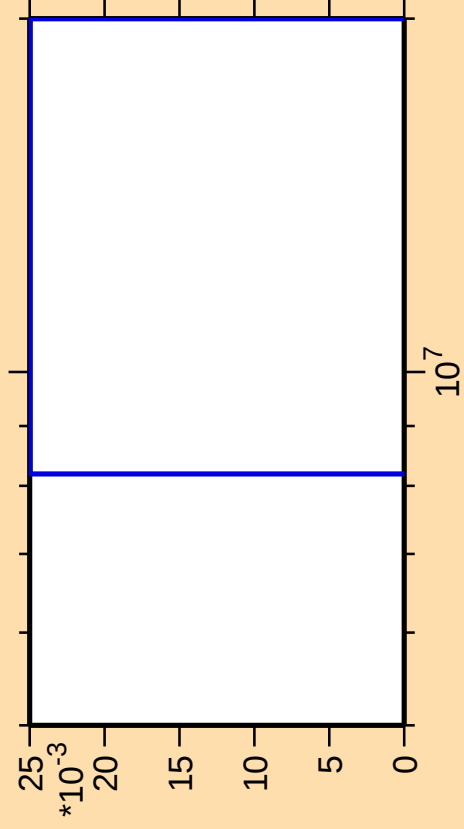
\Delta\sigma/\sigma vs. E for ^{249}\text{Cm}(n,\text{He}3)
