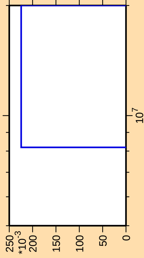
\Delta\sigma/\sigma vs. E for ^{249}\text{Cm}(n,3n\alpha)
