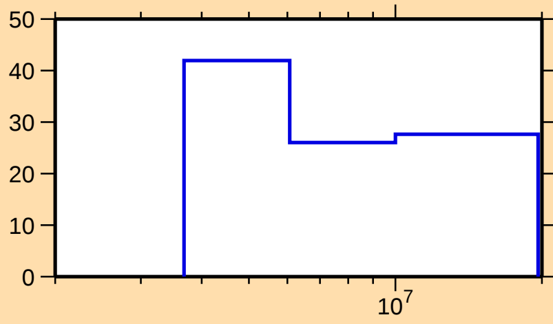
\Delta\sigma/\sigma vs. E for ^{283}\text{Po}
