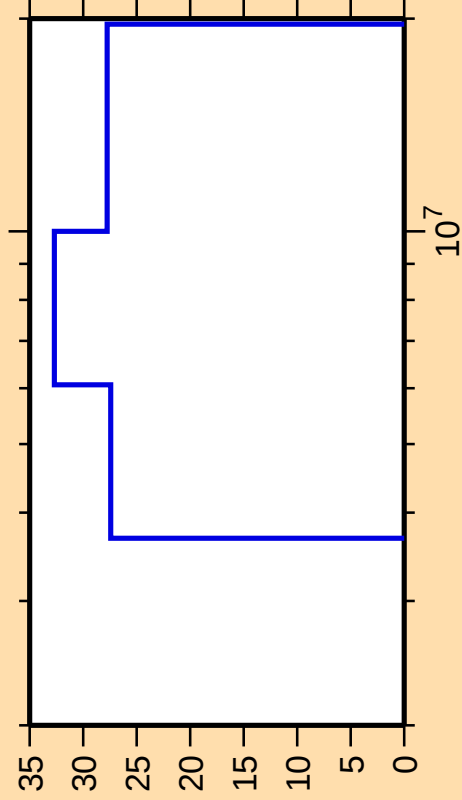
\Delta\sigma/\sigma vs. E for ^{283}\text{Po}
