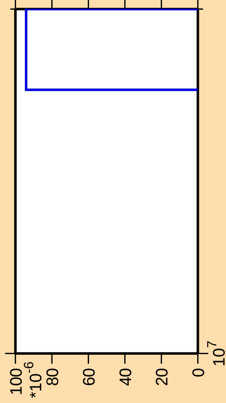
\Delta\sigma/\sigma vs. E for ^{60}\text{Co}(\text{mt } 34)
