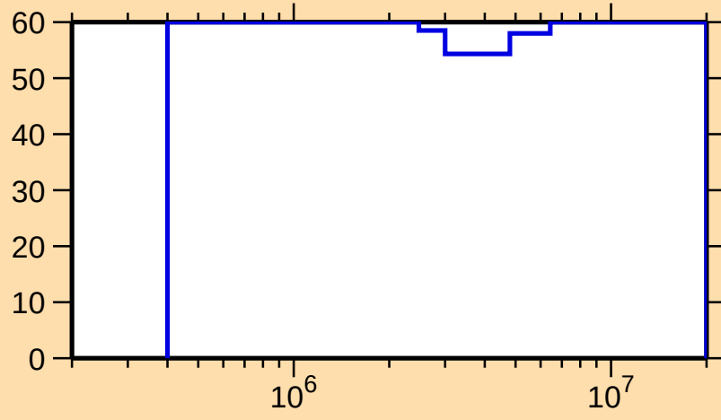
\Delta\sigma/\sigma vs. E for ^{60}\text{Co}(n,\gamma)
