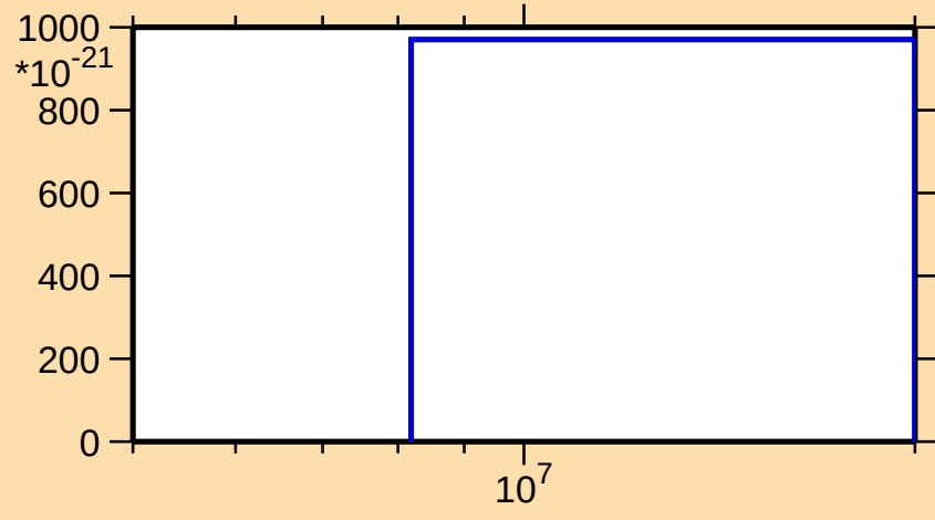
\sigma vs. E for ^{60}\text{Co}(\text{mt } 34)
