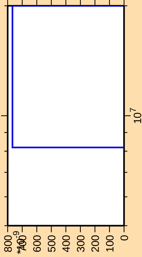
\Delta\sigma/\sigma vs. E for ^{60}\text{Co}(\text{mt } 34)
