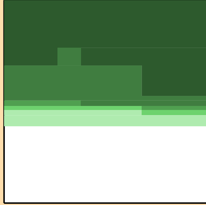
\Delta\sigma/\sigma vs. E for ^{115}\text{Cs}(n,\text{nonel.})
