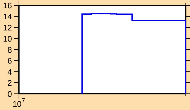
\Delta\sigma/\sigma vs. E for ^{115}\text{Cs}(n,\text{inel.})
