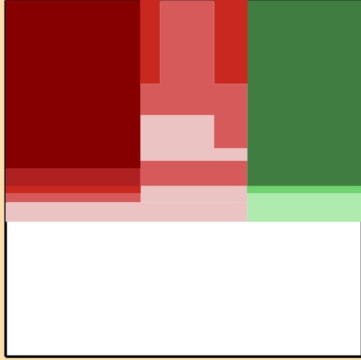
\Delta\sigma/\sigma vs. E for ^{115}\text{Cs}(n,\text{el.})
