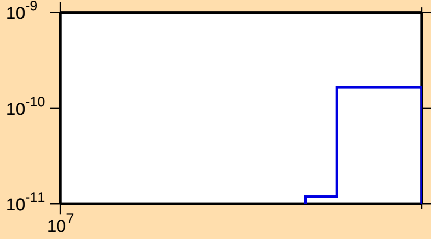
\sigma vs. E for ^{115}\text{Cs}(n,2n\alpha)
