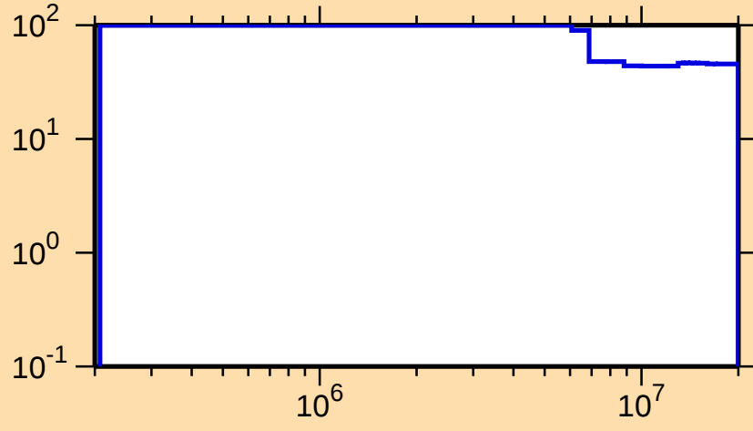
\Delta\sigma/\sigma vs. E for ^{115}\text{Cs}(n,n\text{cont.})
