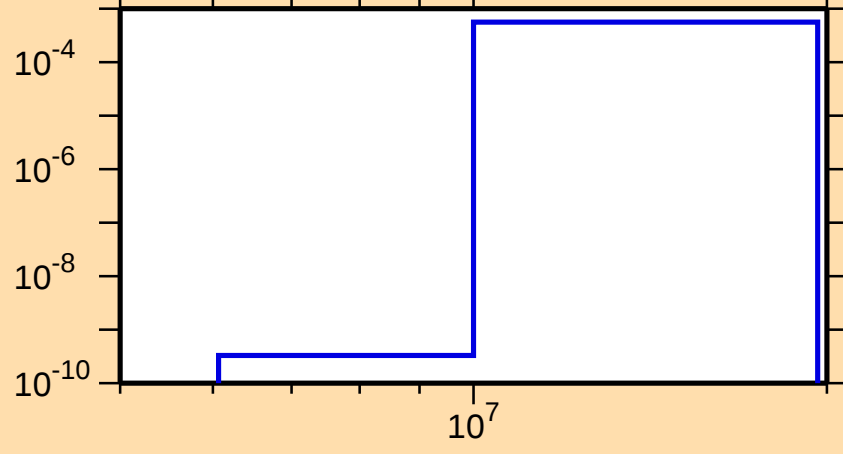
\sigma vs. E for ^{115}\text{Cs}(n,t)
