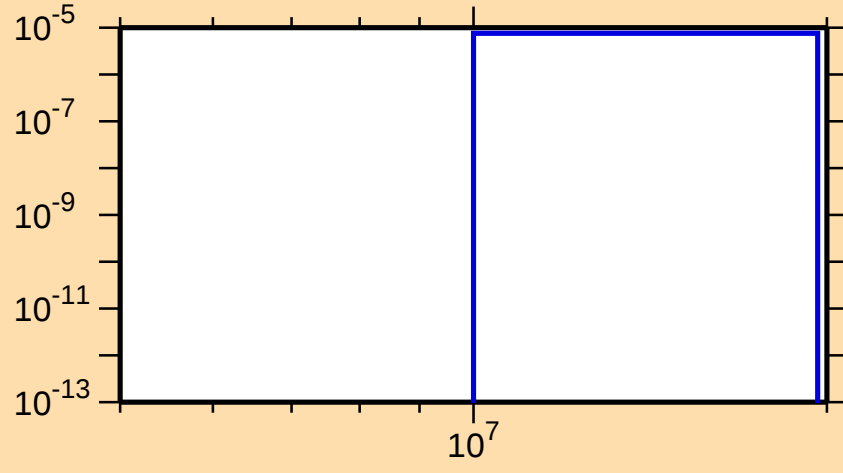
\sigma vs. E for ^{115}\text{Cs}(n,\text{pt})
