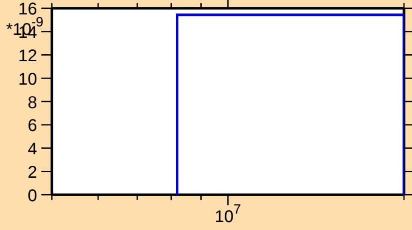
\sigma vs. E for ^{115}\text{Cs}(n,\text{nd})
