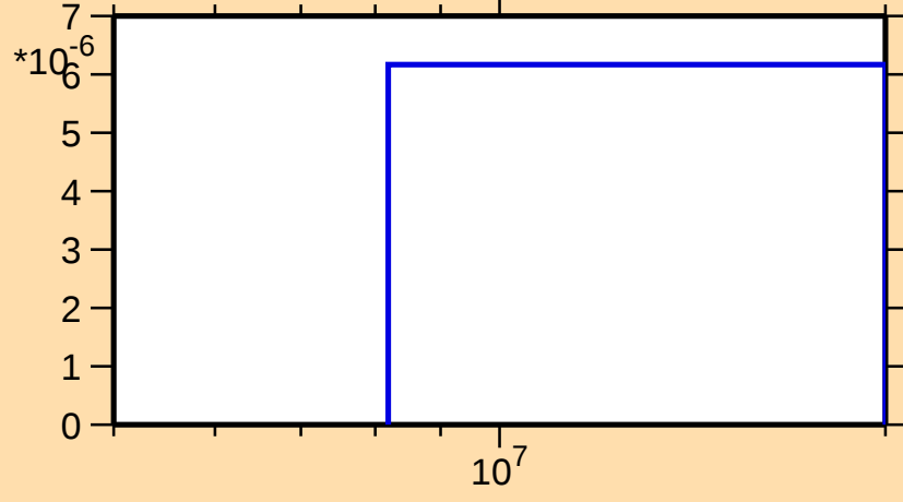
\sigma vs. E for ^{115}\text{Cs}(n,\text{pt})
