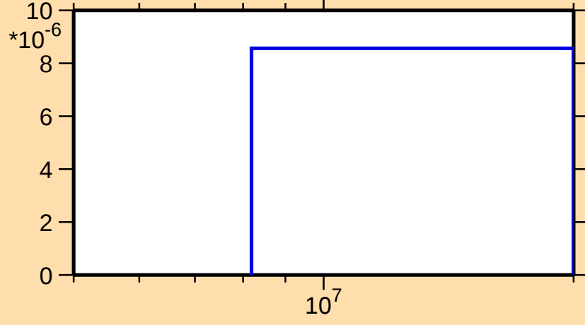
\sigma vs. E for ^{115}\text{Cs}(n,2n)
